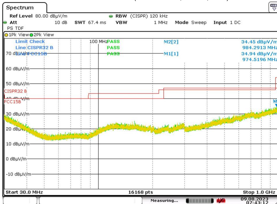
Left Bud – Worst Case (Mid Channel, X-Axis, DH5)
