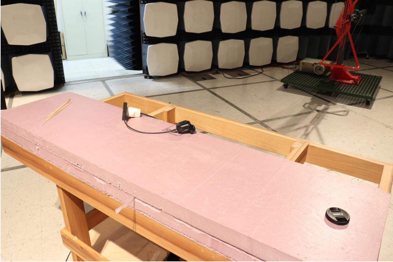
Radiated Emissions 30 MHz to 1 GHz, Charging
