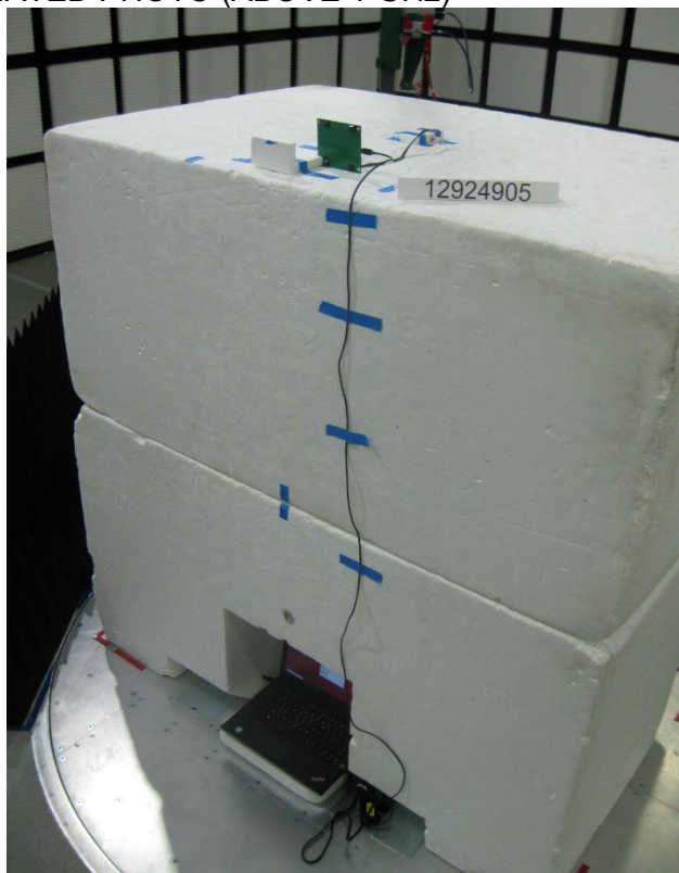
RADIATED PHOTO (ABOVE 1 GHz)
