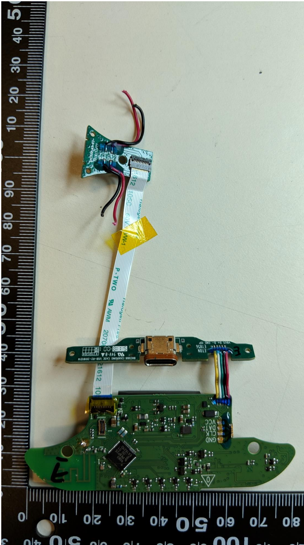
Bose Model 427929 Internal Photos
