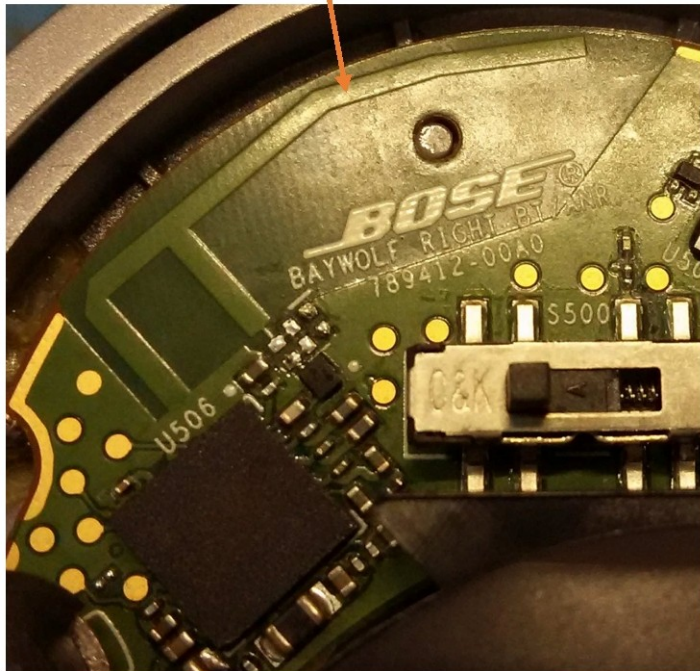
Integrated, printed inverted-F style antenna (no antenna connector present)
