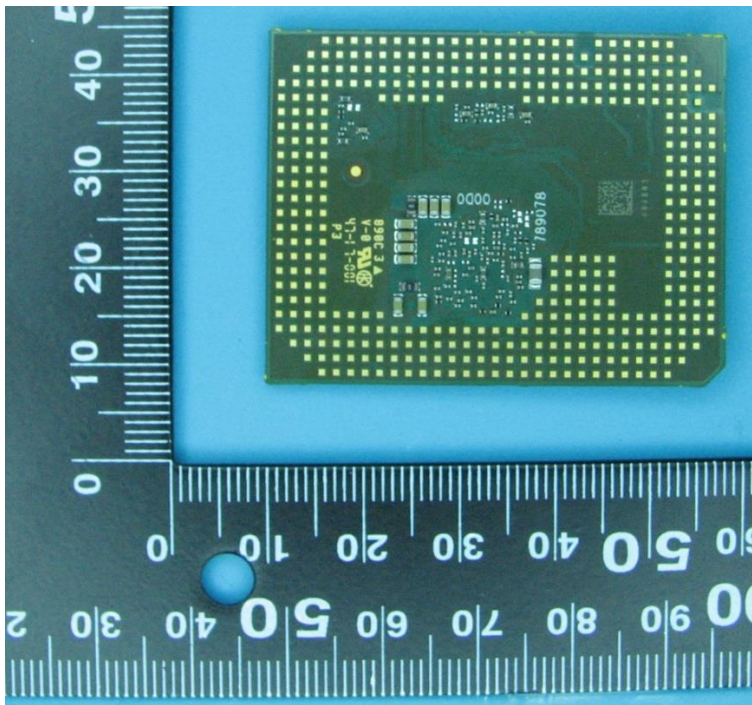
Module bottom view
