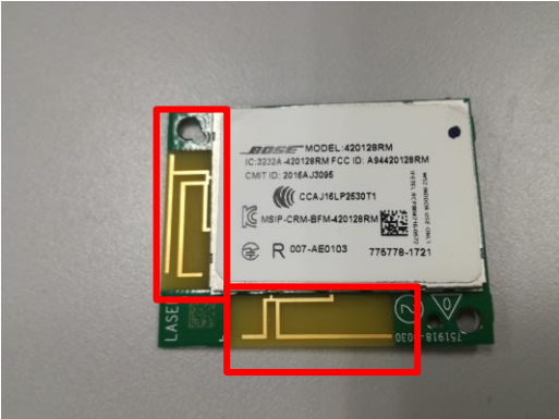
Certified Module 420128RM Antenna Locations
