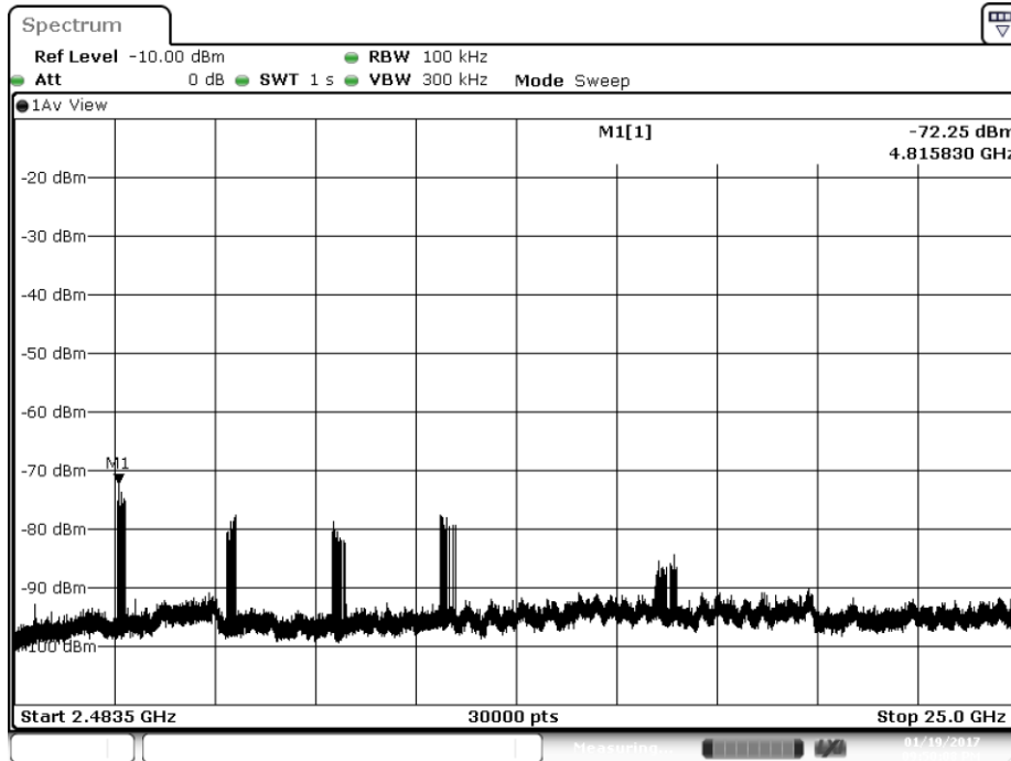
Plot2 DH5 Hopping Average Band 2
