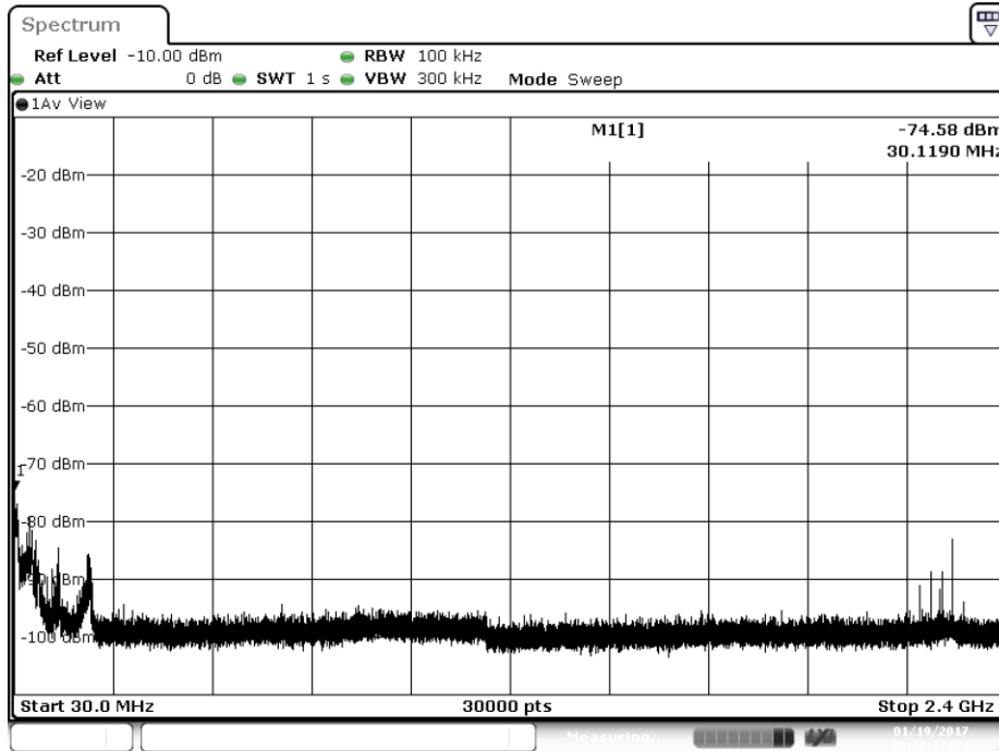
Plot1 DH5 2480 MHz Average Band 1
