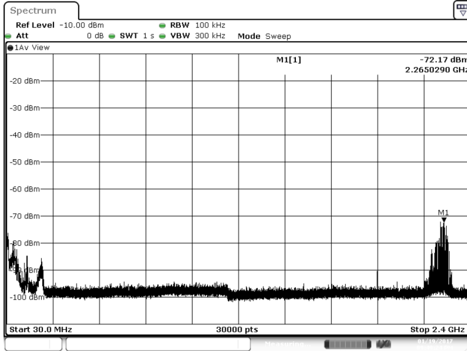
Plot1 DH5 Hopping Average Band 1
