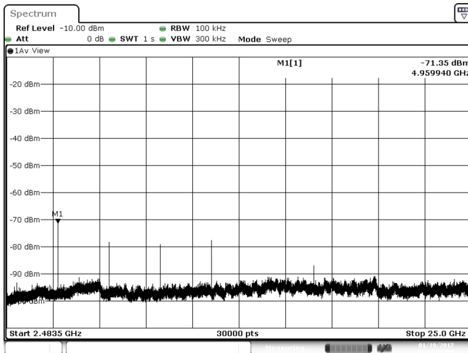
Plot2 DH5 2480 MHz Average Band 2
