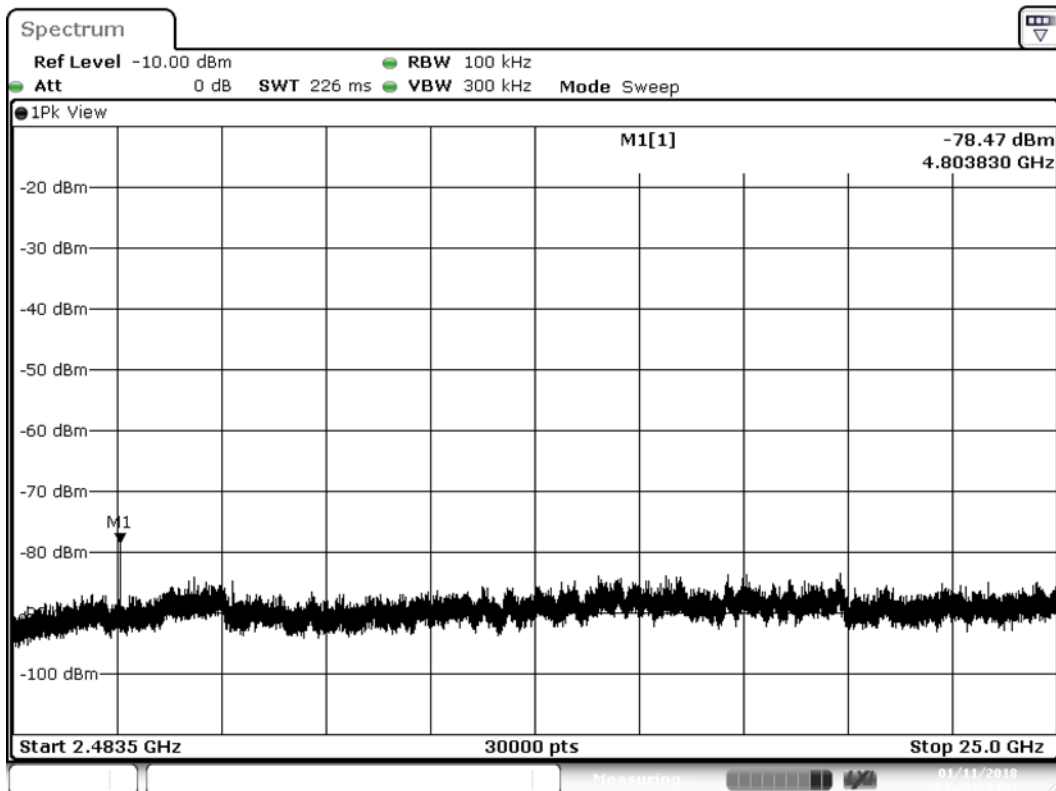
Plot2 BLE 2402 MHz Peak Band 2
