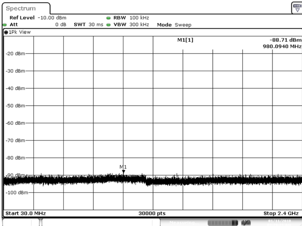
Plot1 BLE 2442 MHz Peak Band 1
