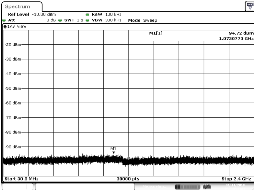
Plot1 BLE 2480 MHz Average Band 1
