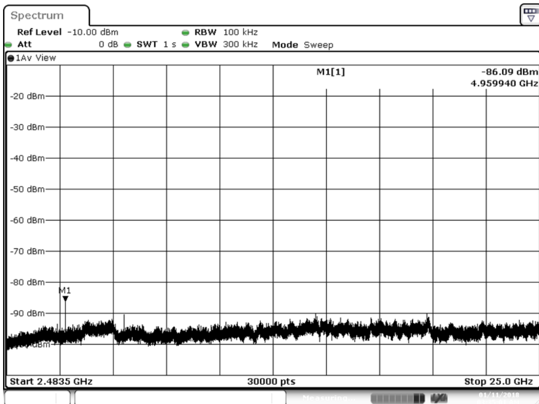
Plot2 BLE 2480 MHz Average Band 2
