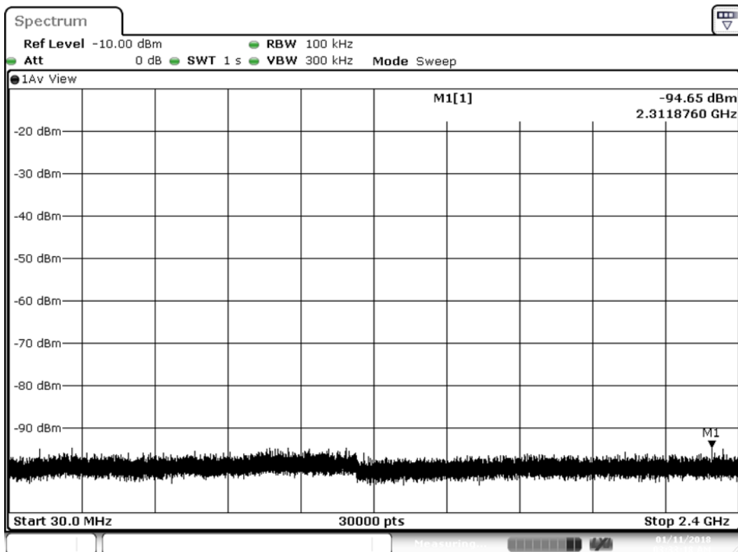
Plot1 BLE 2442 MHz Average Band 1
