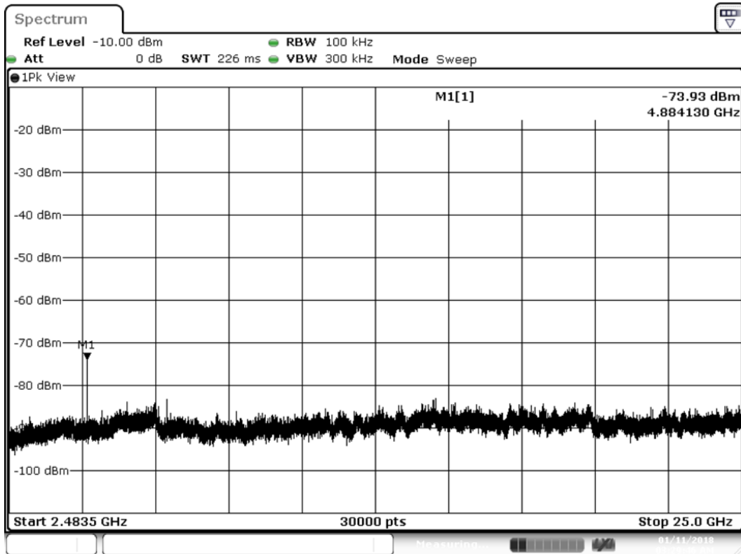
Plot2 BLE 2442 MHz Peak Band 2
