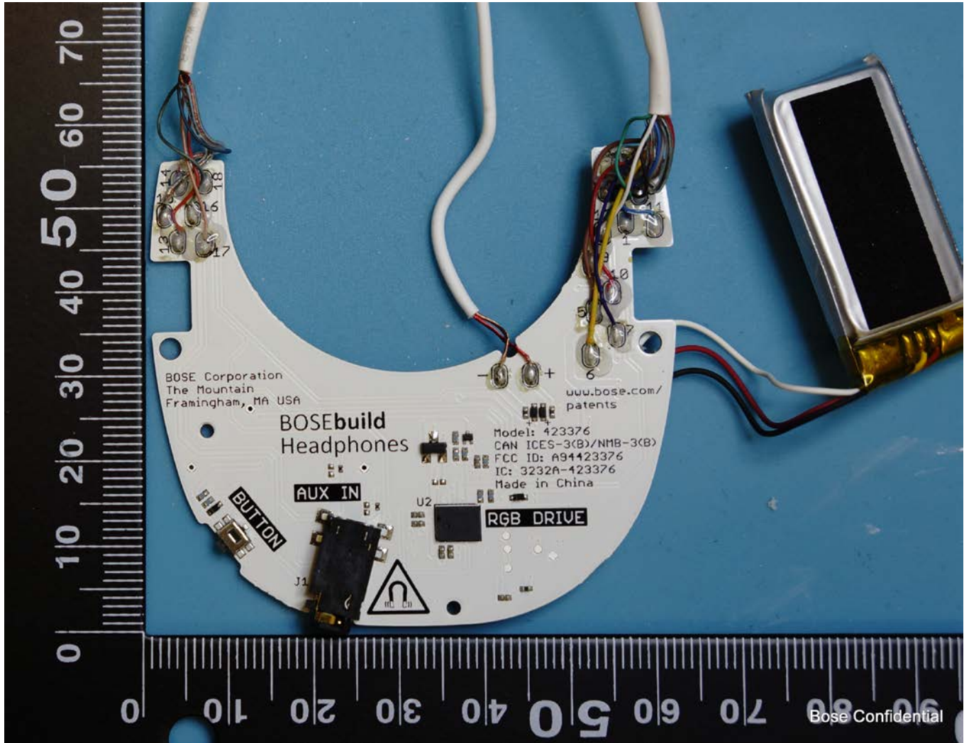
Top side of Left Earcup circuit board showing product labeling
