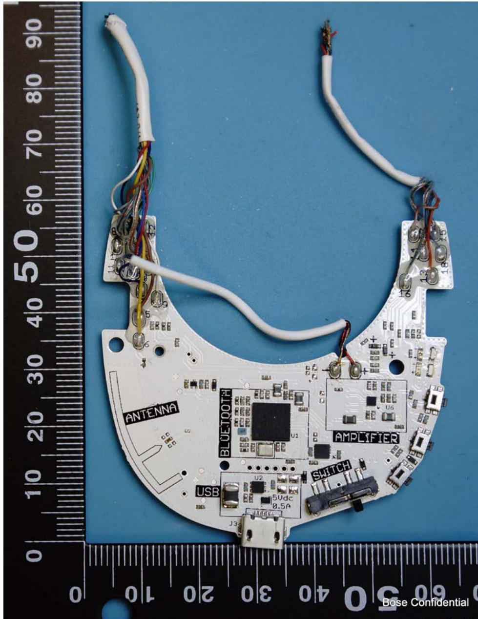
Right Earcup circuit board showing antenna location under solder mask.
