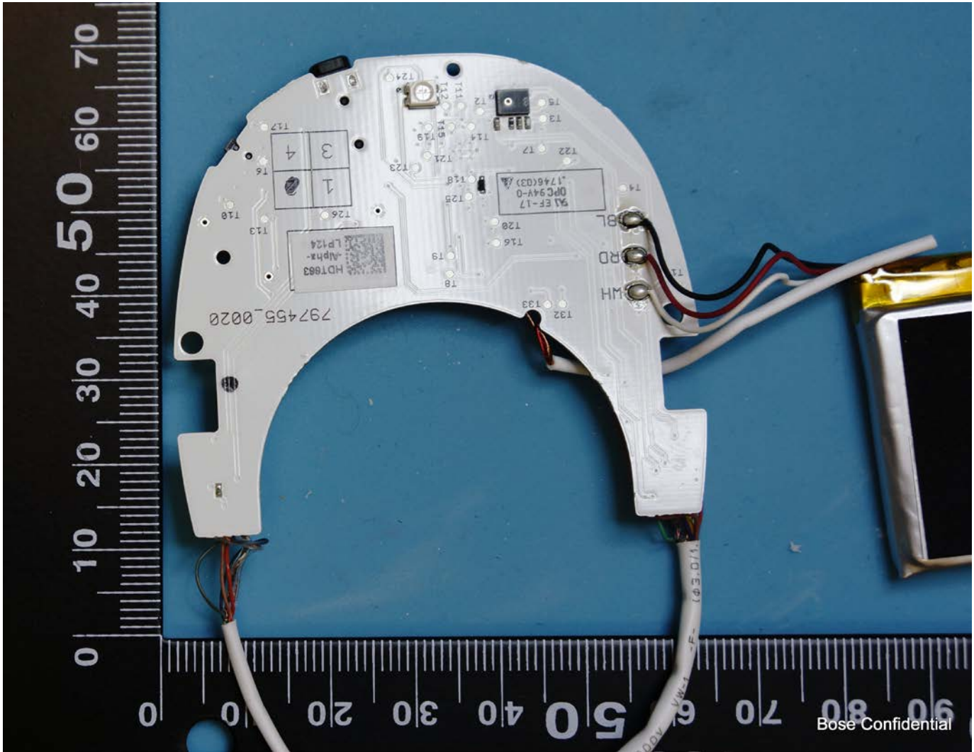
Bottom side of Left Earcup circuit board
