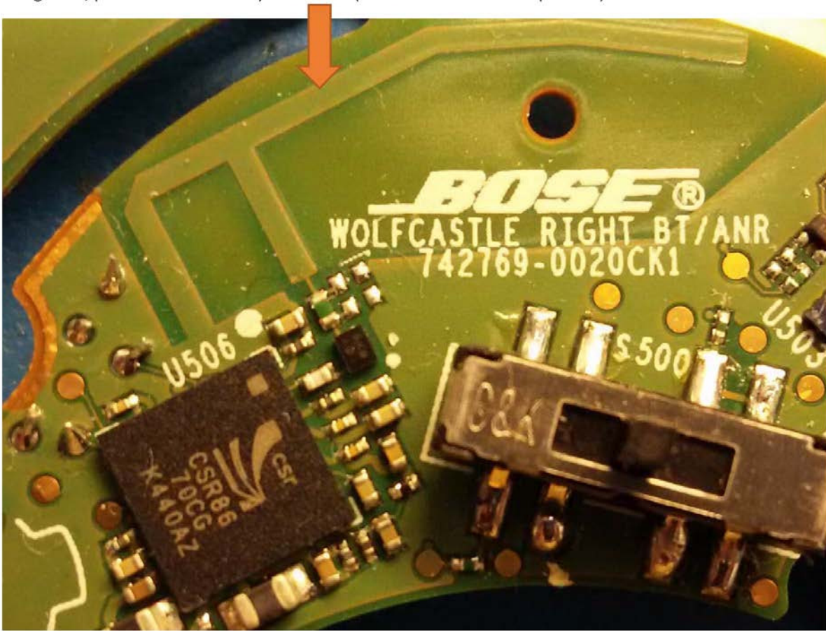
Zoomed in view of Radio PCB, w/ Antenna
