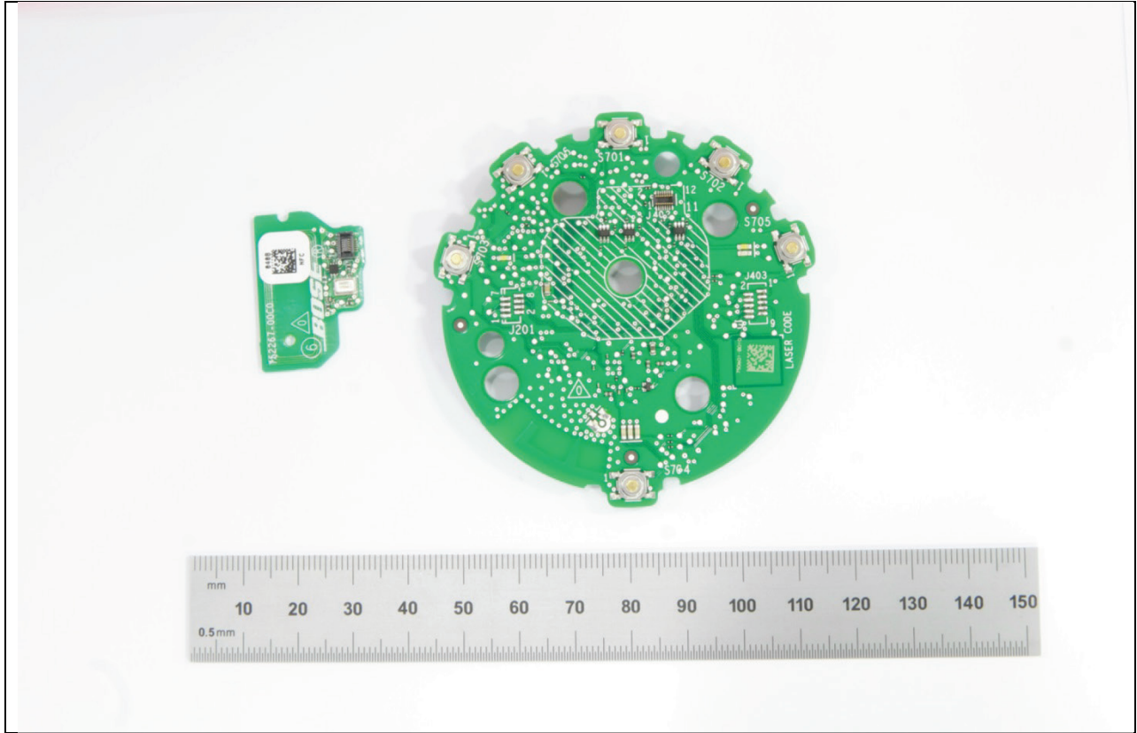
Control (Radio) Board (Top)
