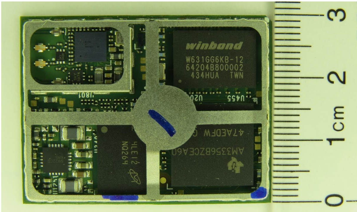
Module solder side
