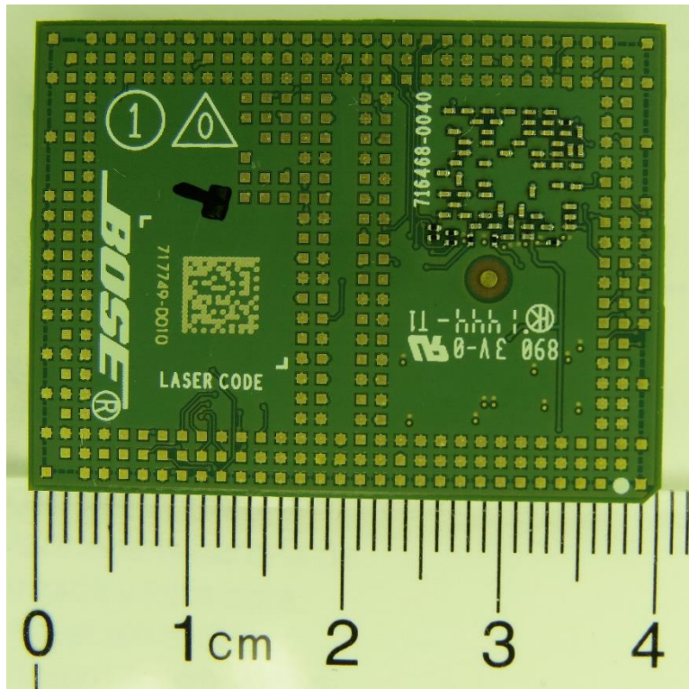
Module solder side
