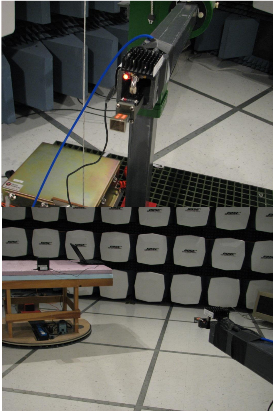
Radiated emissions 18 GHz to 26 GHz, 3 meter distance.
