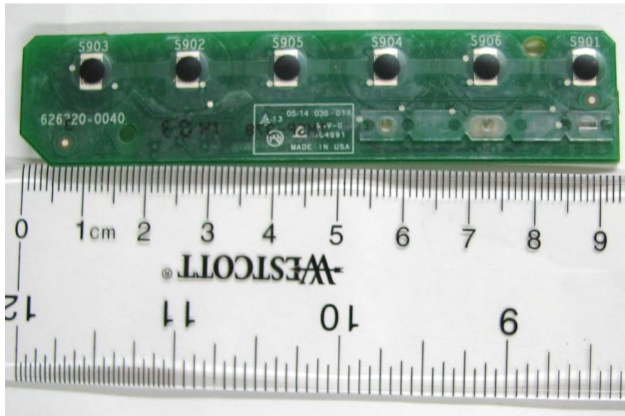
Button PCB bottom side
