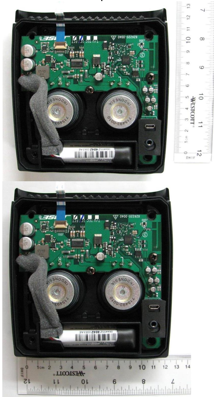
Main PCB component side.
