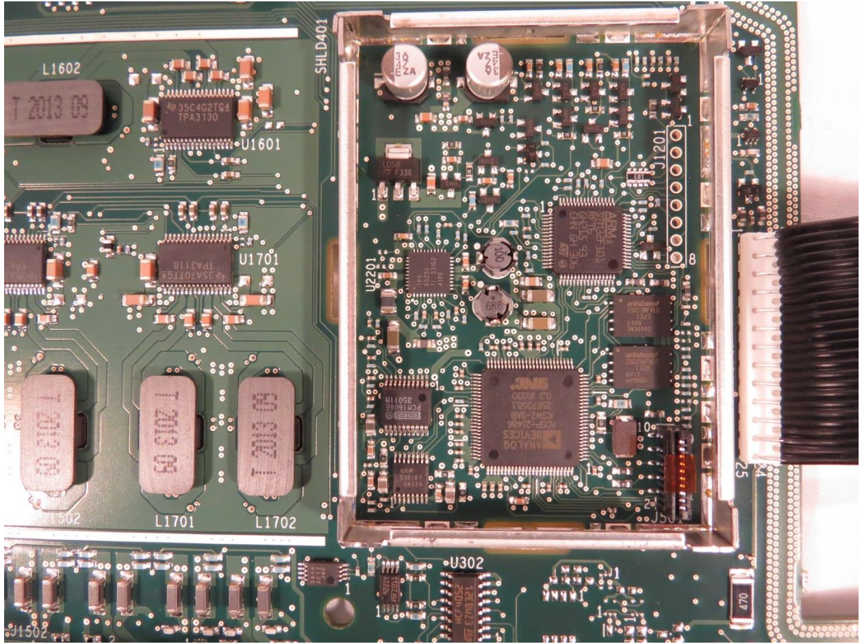
Main Board Close-ups Processing (Top)
