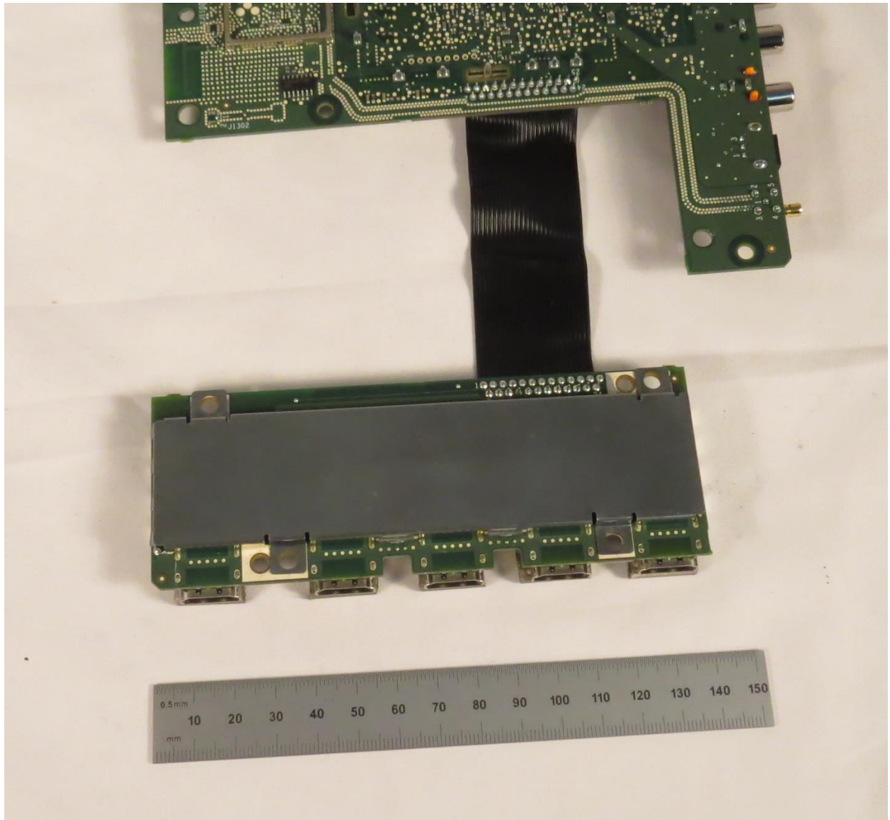
Mezzanine Board Bottom
