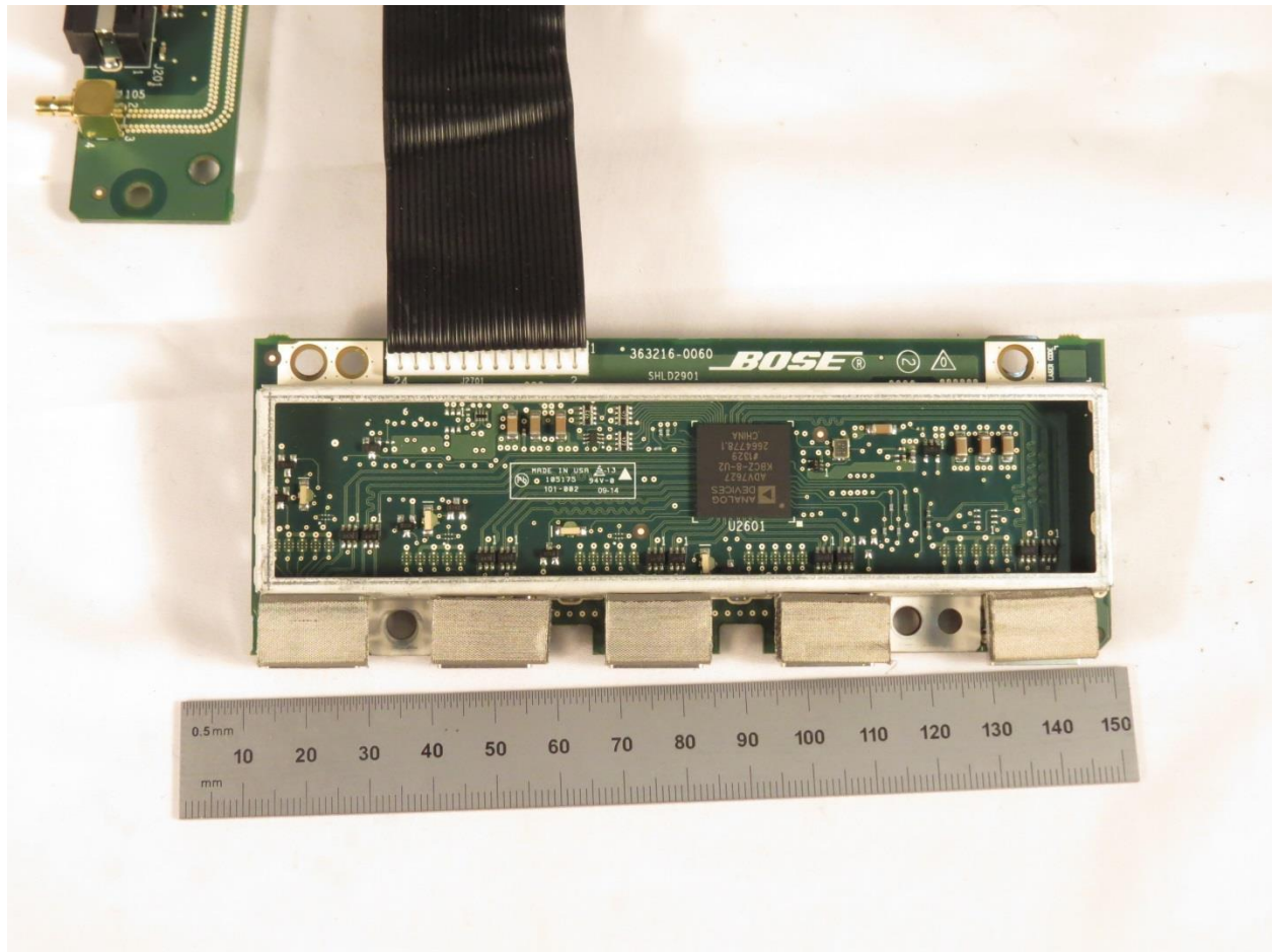
Mezzanine Board Top
