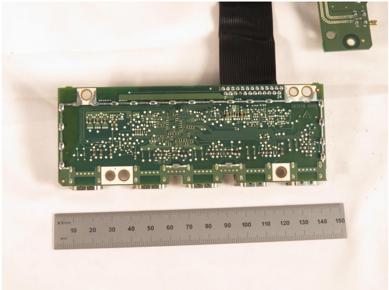
Mezzanine Board Bottom
