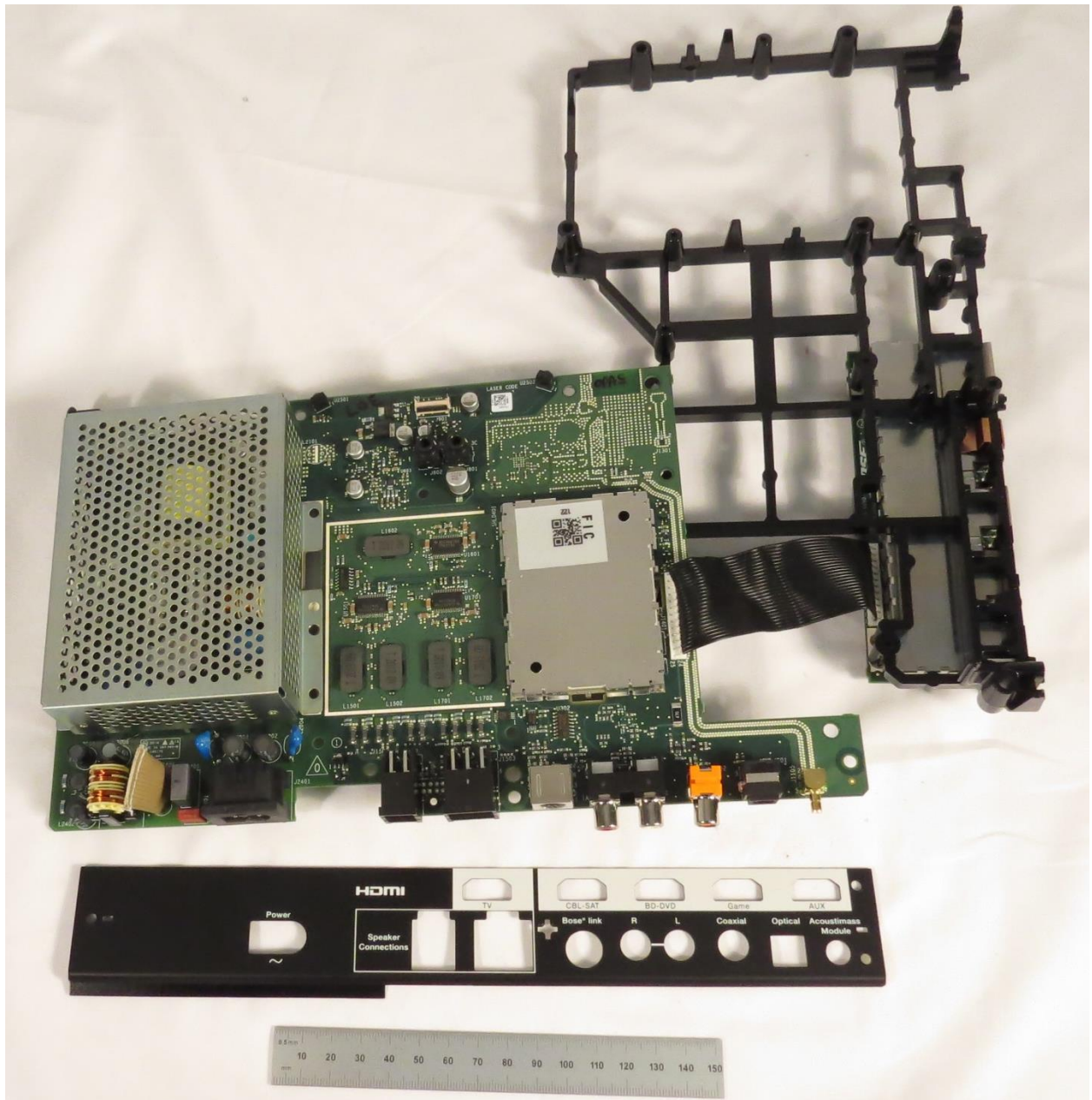
Open Top Partial Disassembly
