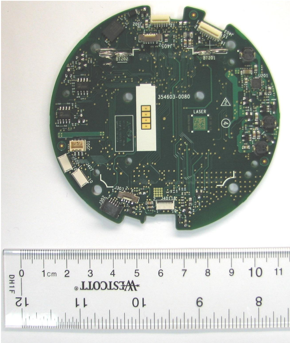
Bottom view with battery label removed
