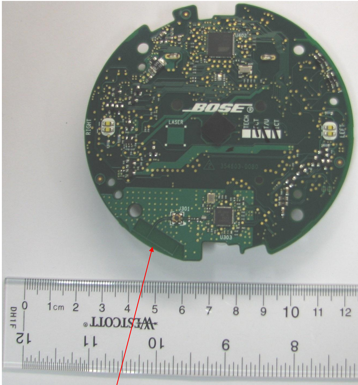
Antenna (printed etch inverted F)
