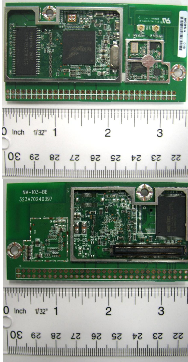
RF module with shields removed
