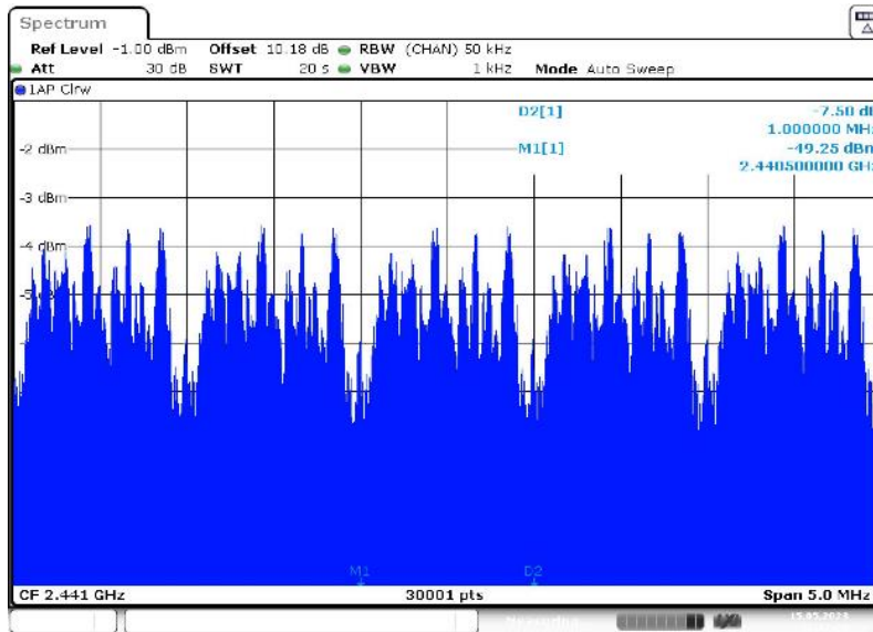
3-DH5 hopping
