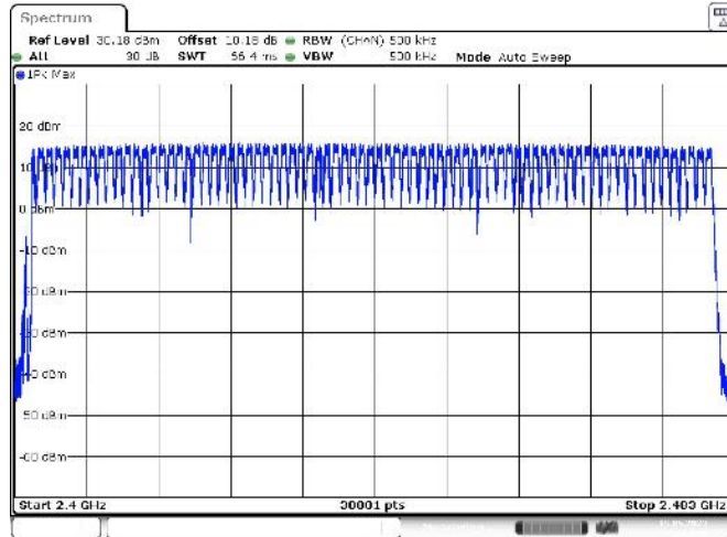
79 hopping channels active DH5
