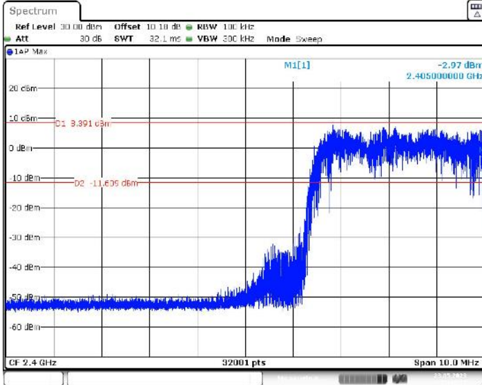
3DH5 low channel band-edge while hopping
