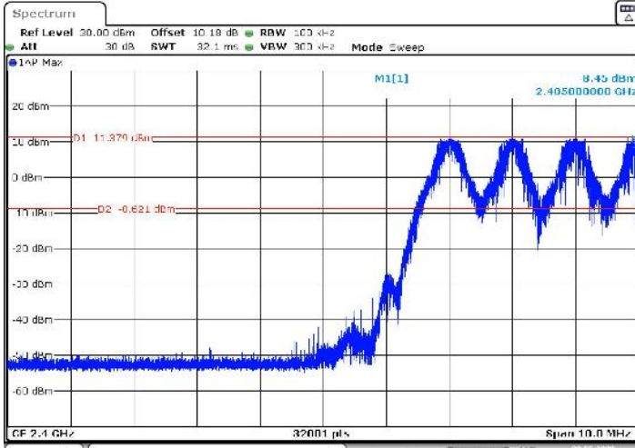
DH5 low channel band-edge while hopping
