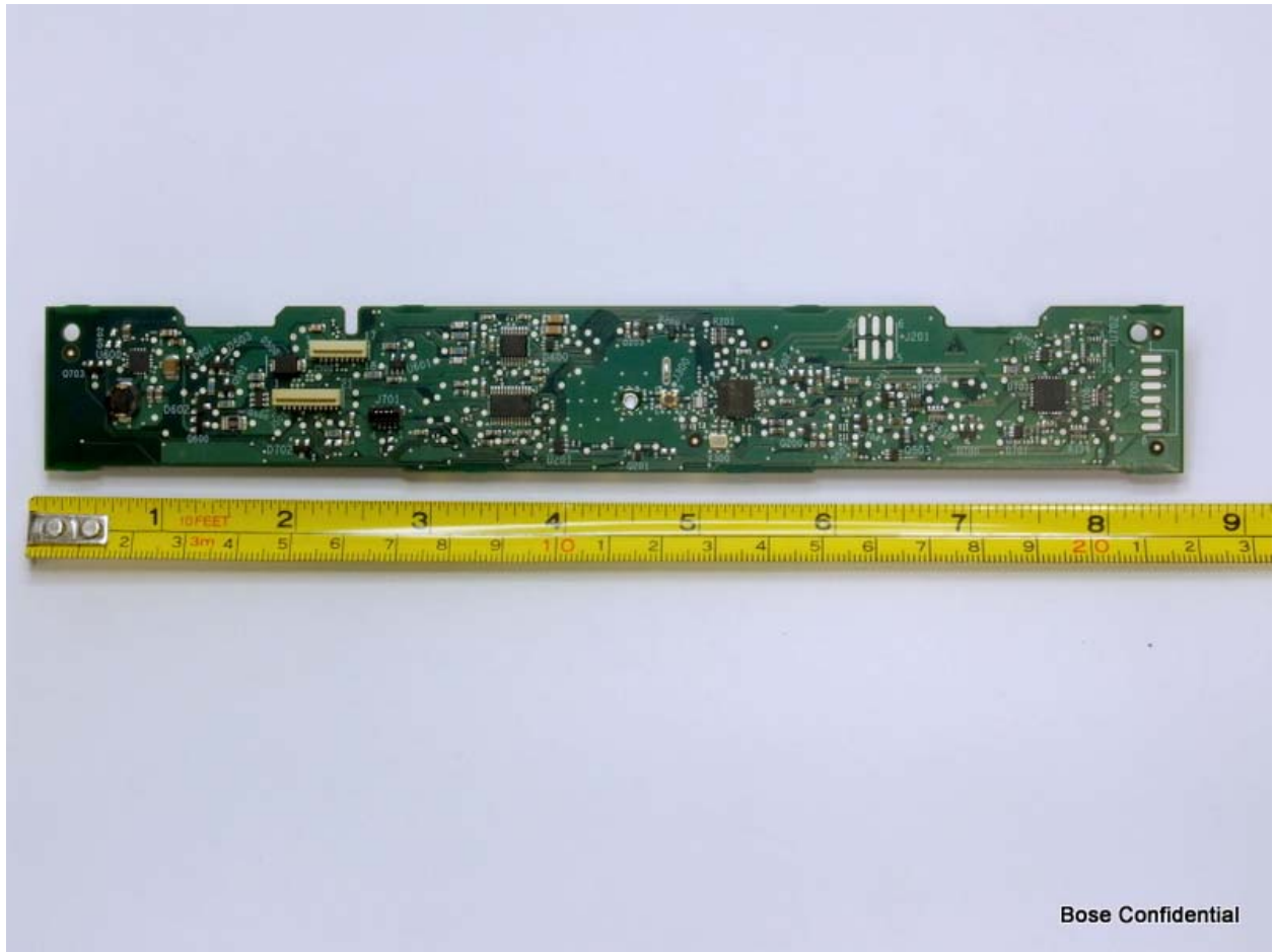
DSP/Radio board bottom side
