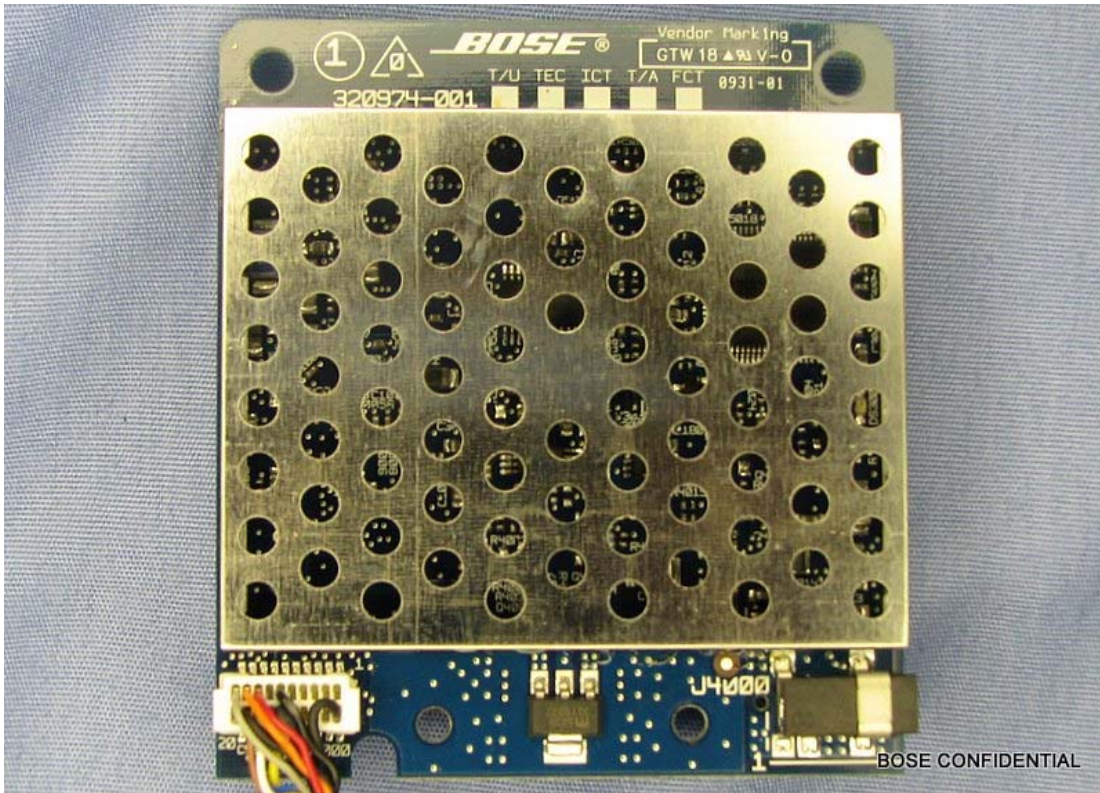
Right side interior with and without shield cover.
