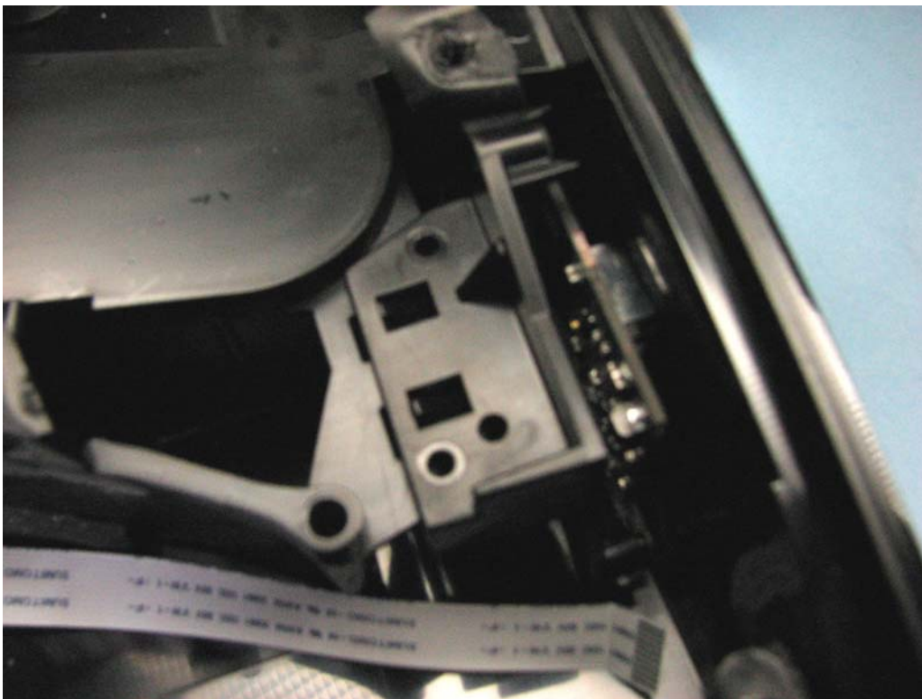
Location of the Bluetooth board
