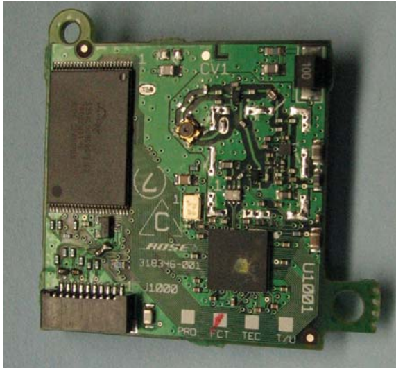
Component side
