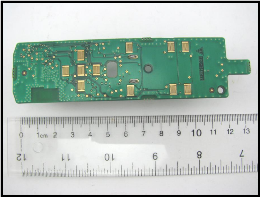
Bottom side (No RF circuitry on this side of the PCB)
