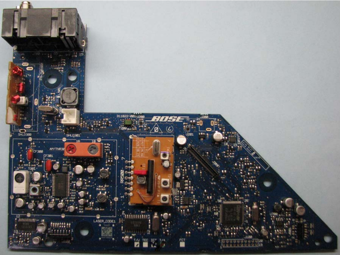
Aux board – shields removed
