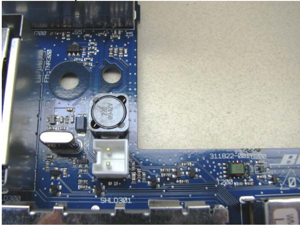
27 MHz TX section – bottom of board
