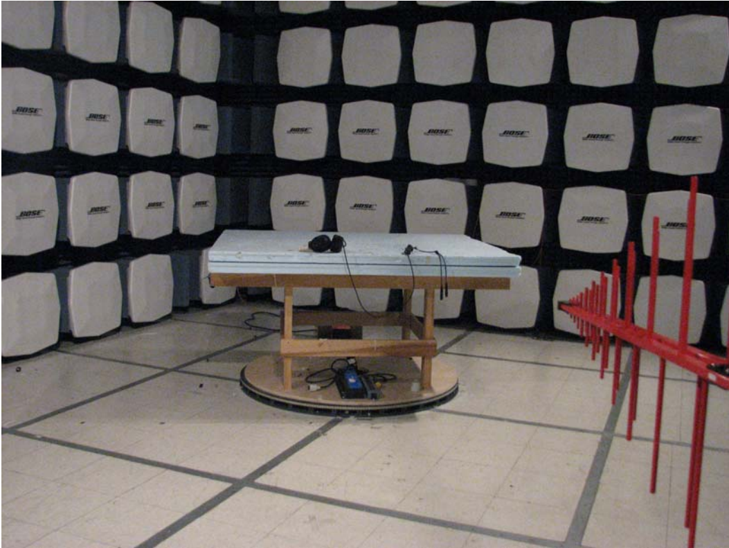
Test setup photos Radiated emissions – 30MHz – 4GHz
