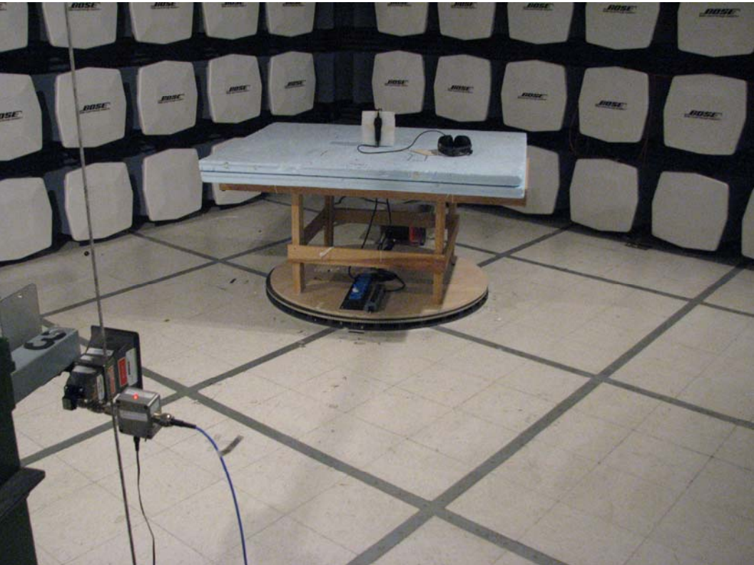
Radiated emissions – 8GHz – 18GHz
