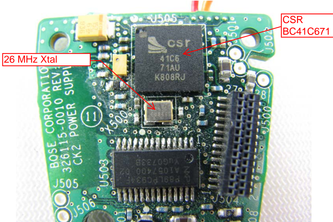
RF PCB top side close up
