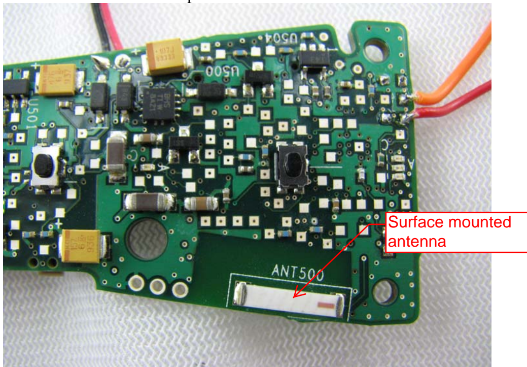
RF PCB bottom side close up
