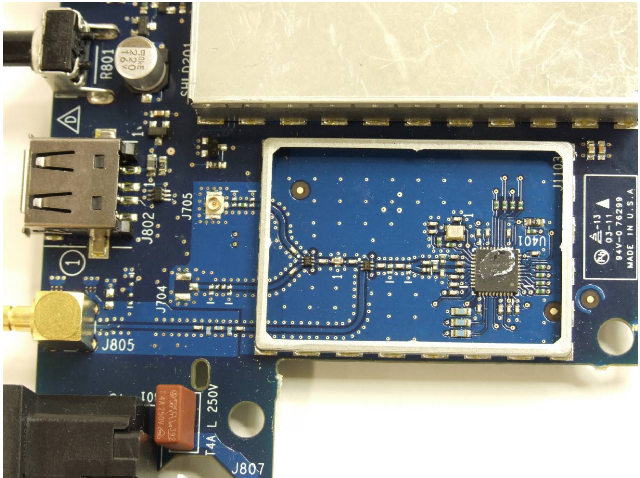
DSP/Radio detail with top with cover removed
