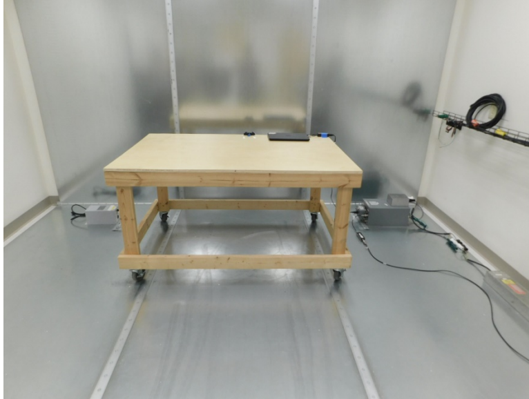
AC LINE CONDUCTED PHOTO
