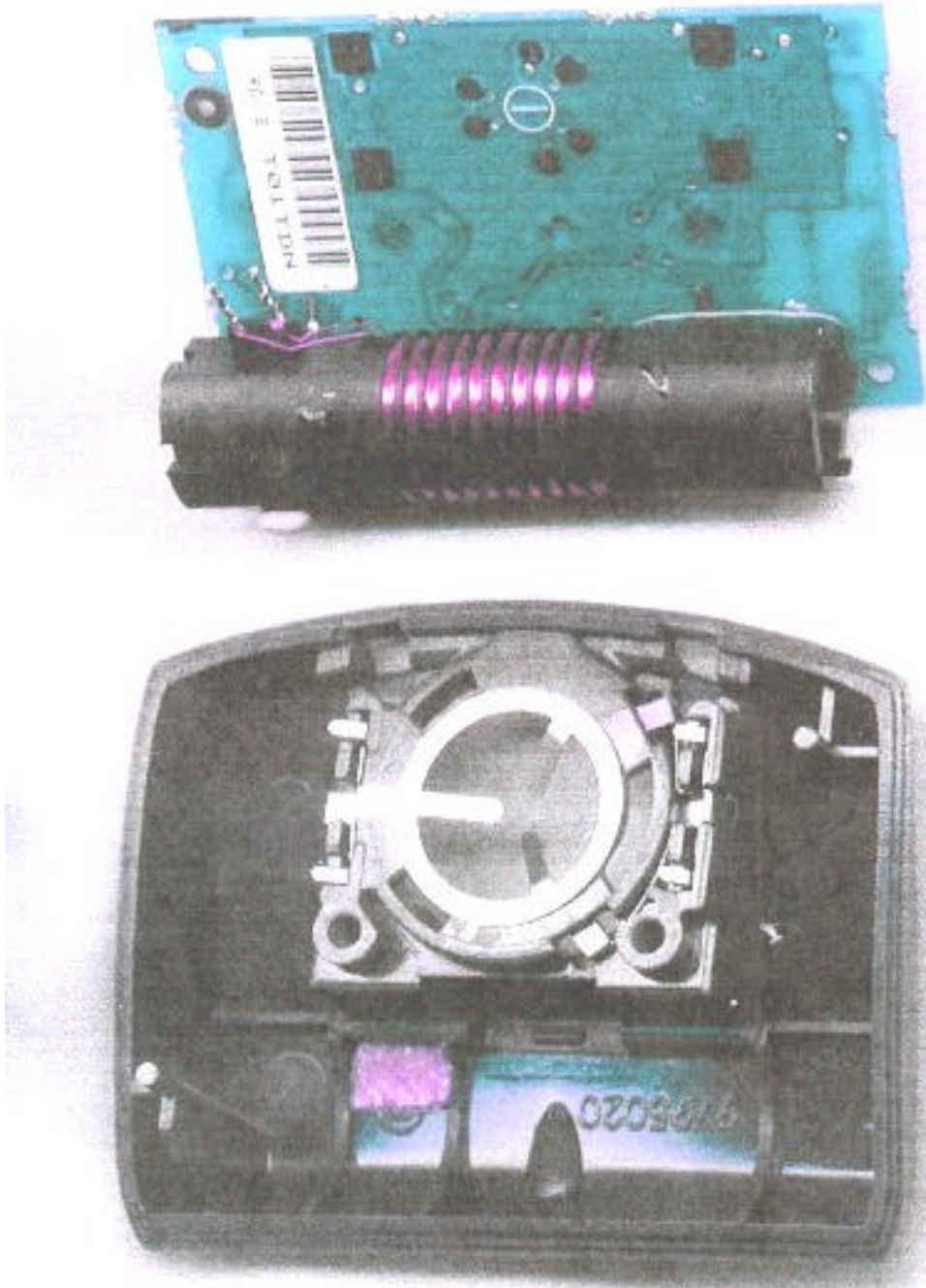
Fig 5. Transponder PCB Assembly Bottom
