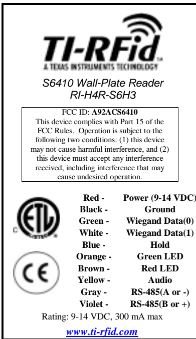
Figure 1. Wall Plate Product Label
