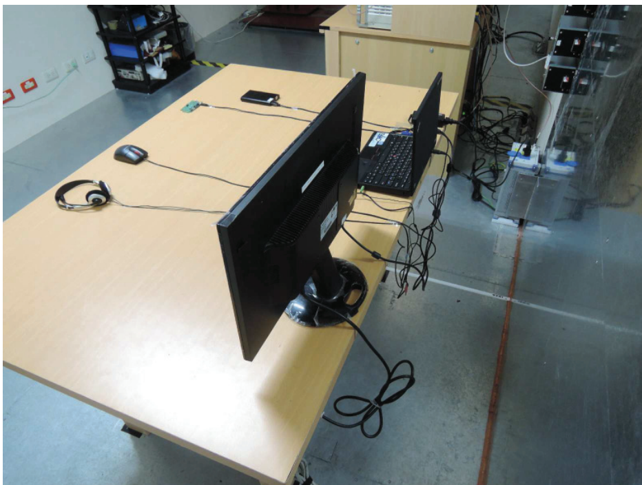
Photograph 5: Set-up for for Mains Conducted testing Back
