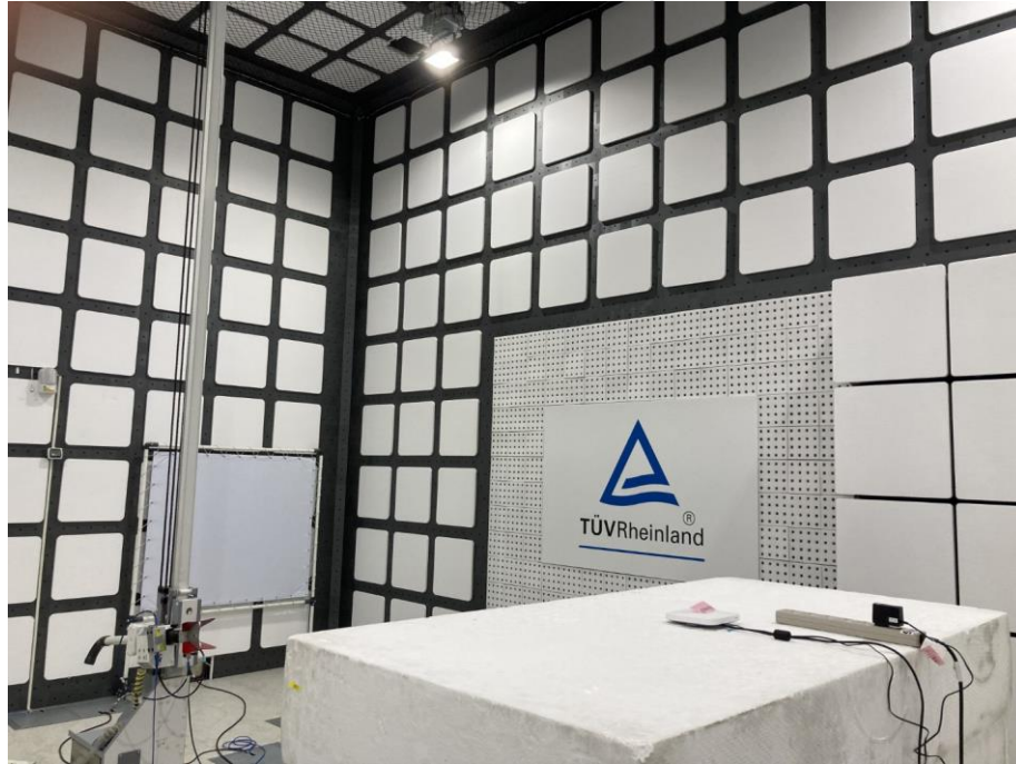
Photograph 18: Test Setup for Spurious Emissions (Back View 4, Adapter Mode)
