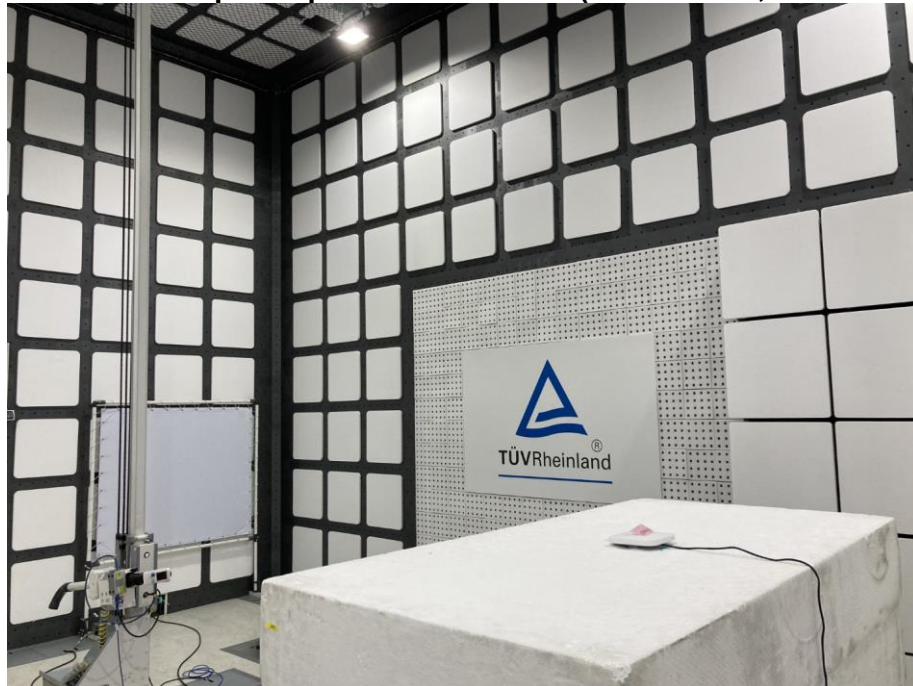
Photograph 24: Test Setup for Spurious Emissions (Back View 4, POE Mode)
