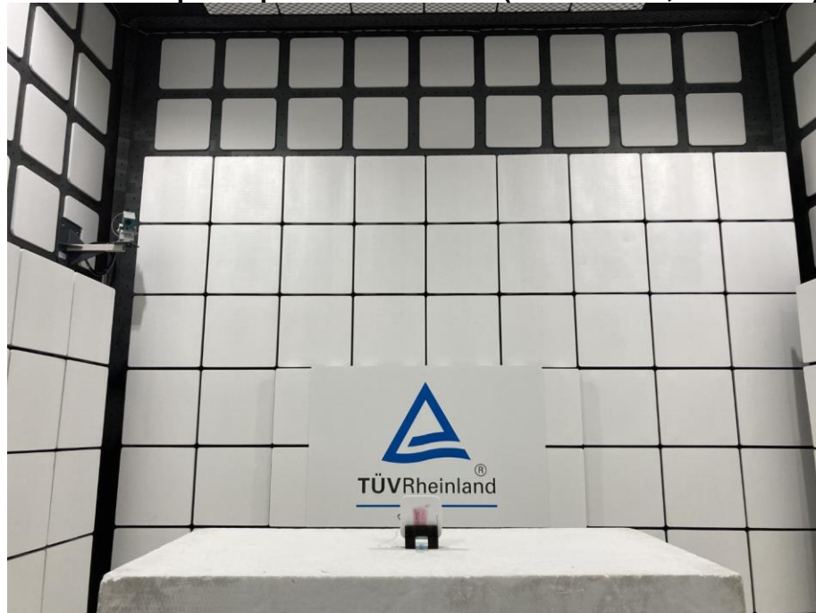
Photograph 8: Test Setup for Spurious Emissions (Front View 2, POE Mode)
