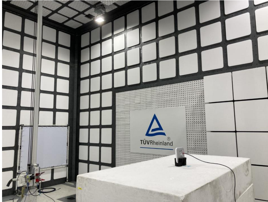
Photograph 12: Test Setup for Spurious Emissions (Back View 4, POE Mode)
