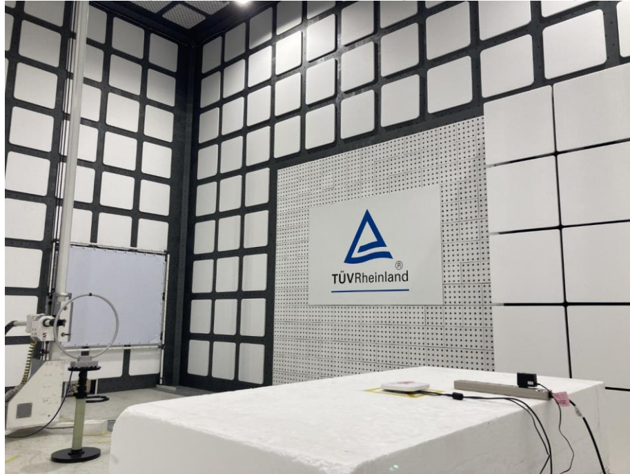
Photograph 16: Test Setup for Spurious Emissions (Back View 2, Adapter Mode)
