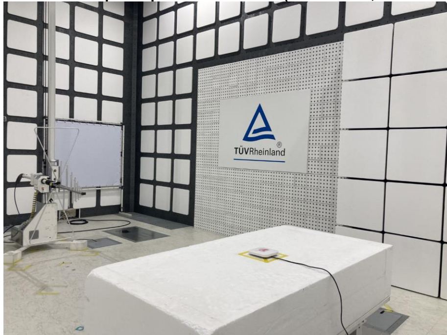
Photograph 22: Test Setup for Spurious Emissions (Back View 2, POE Mode)
