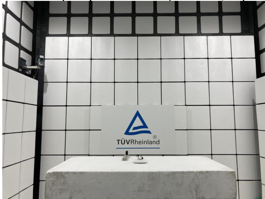
Photograph 14: Test Setup for Spurious Emissions (Front View 2, Adapter Mode)
