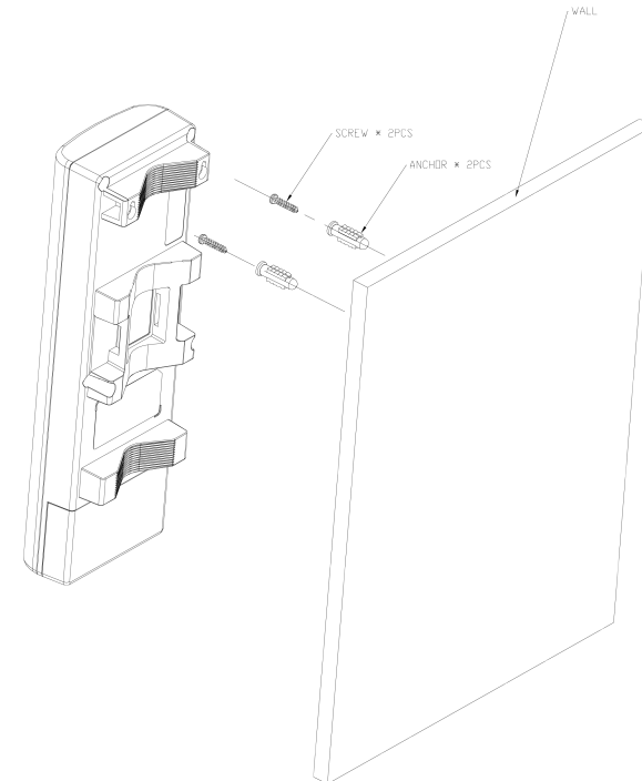
Figure 2-2: Wall Mouting the ENH500
