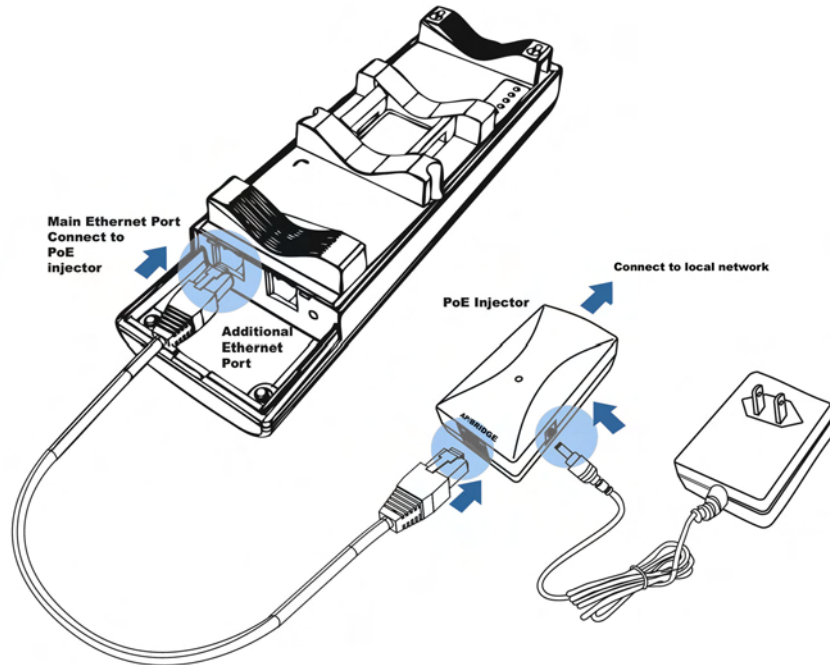
Figure 2-1: Installing the ENH202
