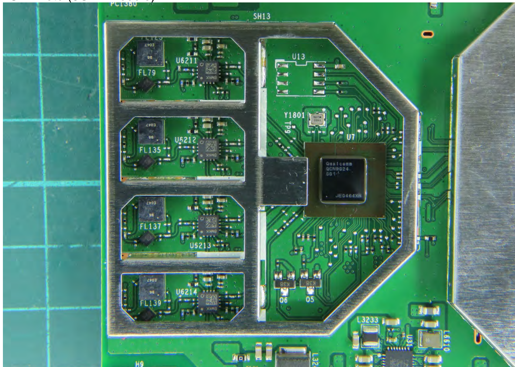
(16) EUT Photo (6GHz Module)
