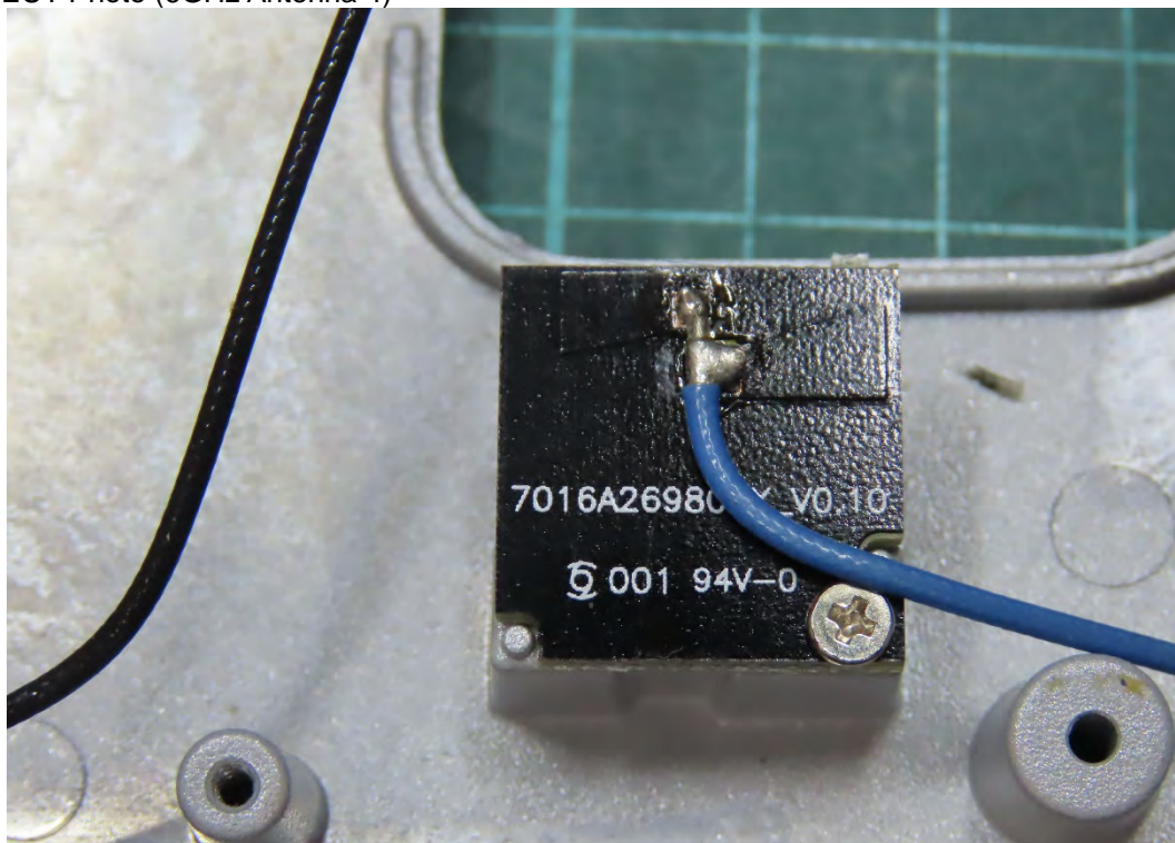
(37) EUT Photo (6GHz Antenna 4)
