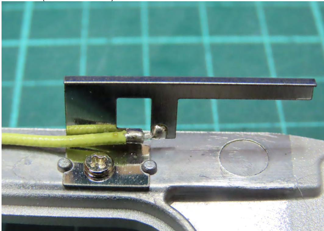
(22) EUT Photo (2.4GHz Antenna 3)
