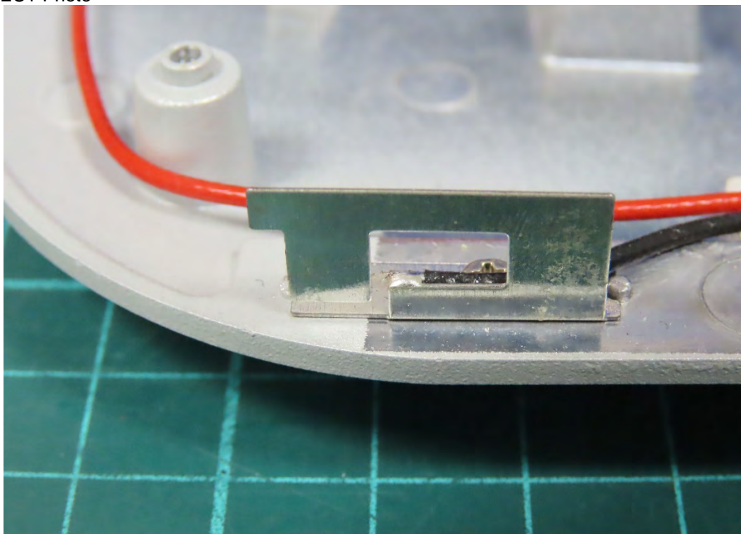
(34) EUT Photo (6GHz Antenna 1)
