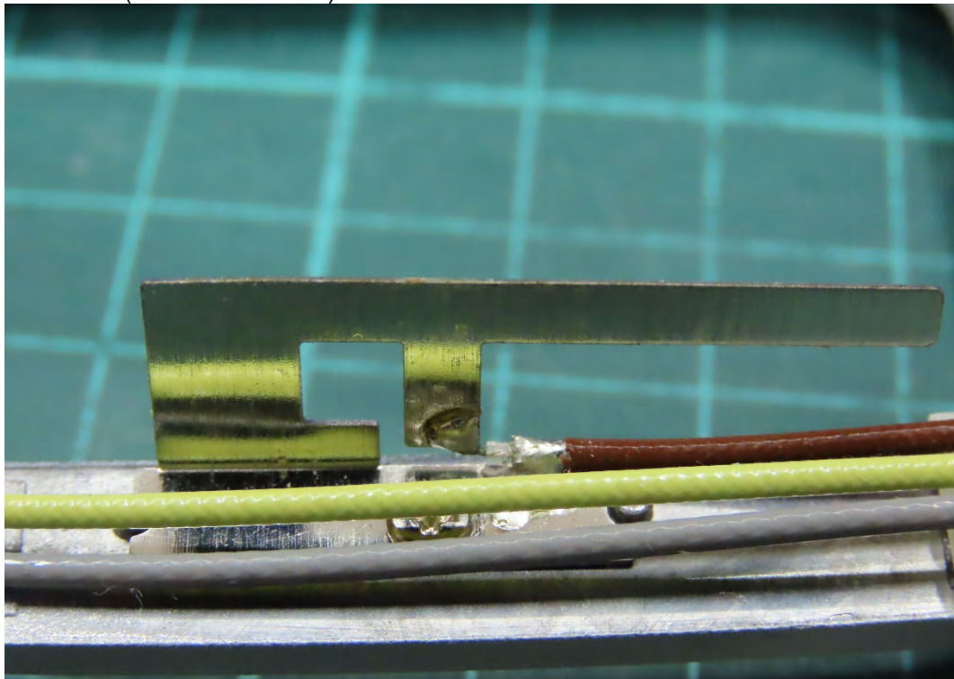
(20) EUT Photo (2.4GHz Antenna 2)
