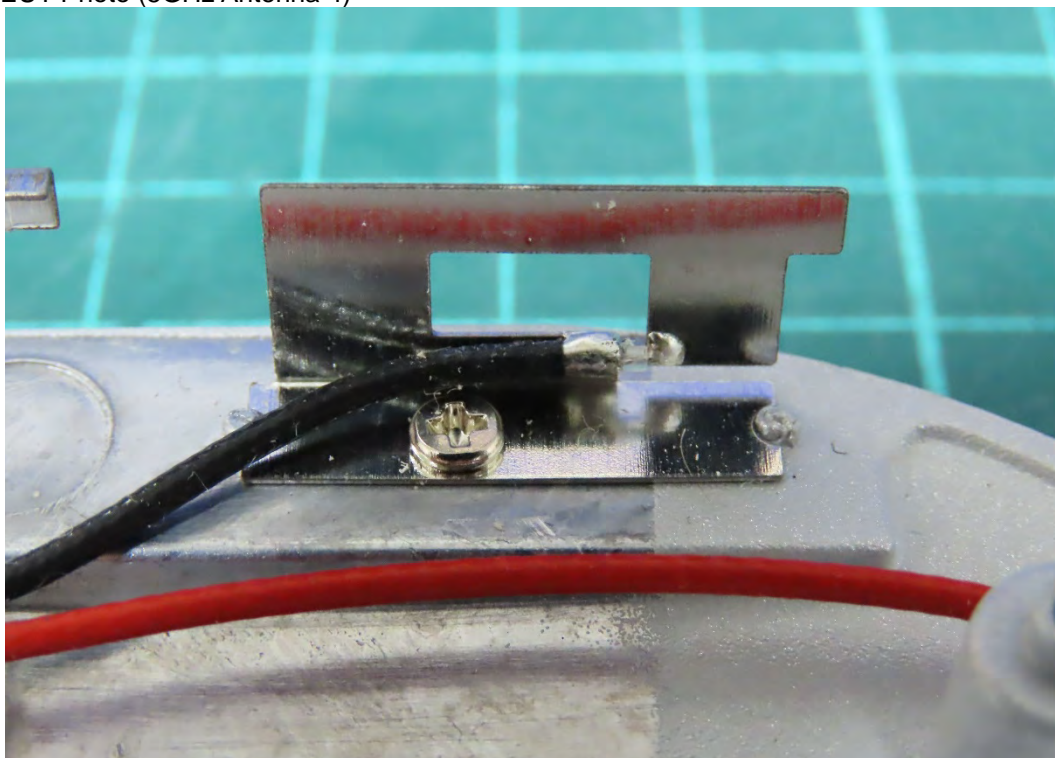
(32) EUT Photo (5GHz Antenna 4)
