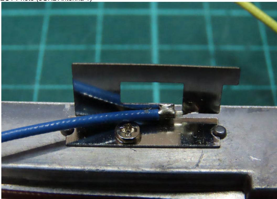
(26) EUT Photo (5GHz Antenna 1)
