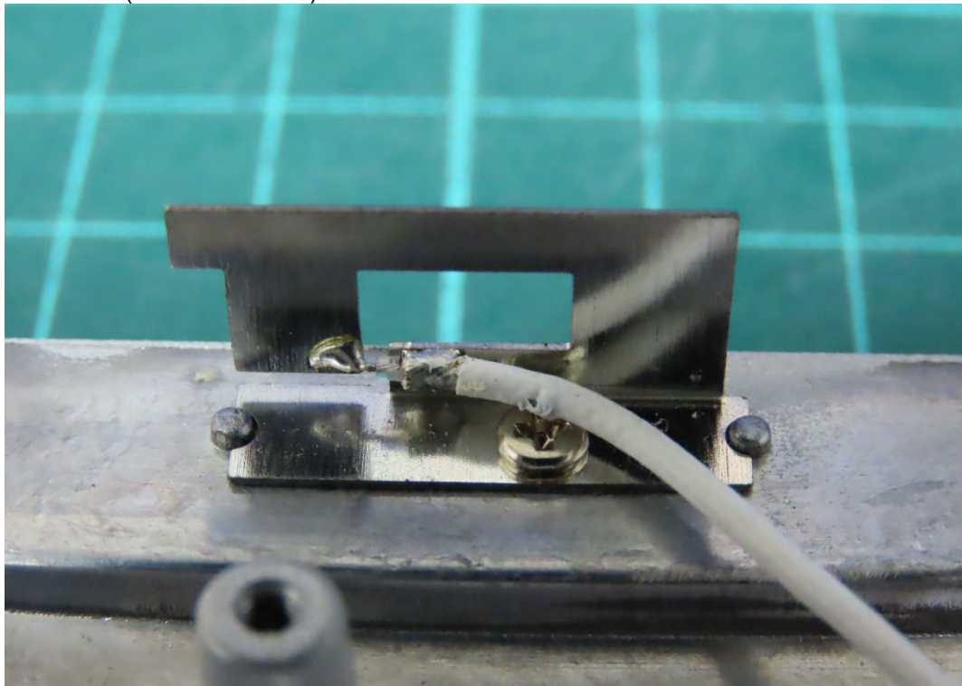
(30) EUT Photo (5GHz Antenna 3)
