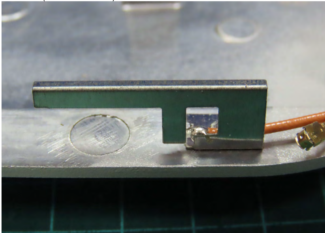
(18) EUT Photo (2.4GHz Antenna 1)
