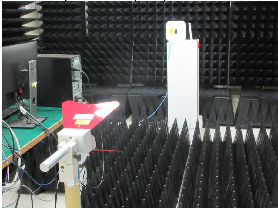
Photograph 18: Test Setup for DFS Mode (View 2)
