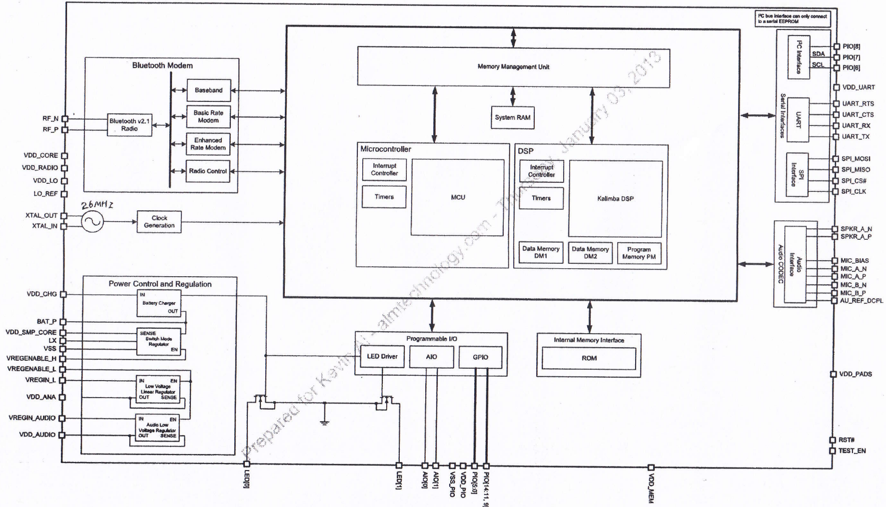
Figure 2.1: BlueCore5-Multimedia ROM QFN Device Diagram
