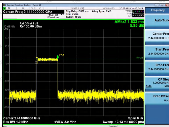
3DH3-Ant1-Hop-PASS
