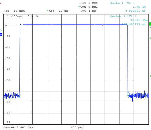
DH5 on time (One Pulse) Plot on Channel 39
