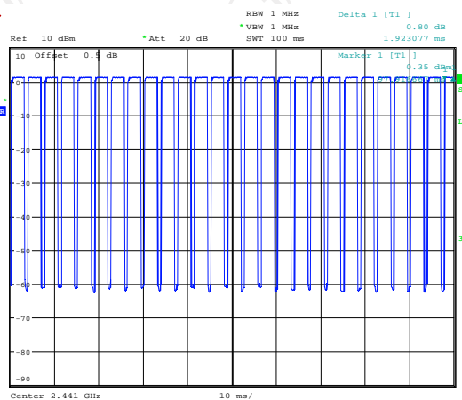
DH5 on time (Count Pulses) Plot on Channel 39
