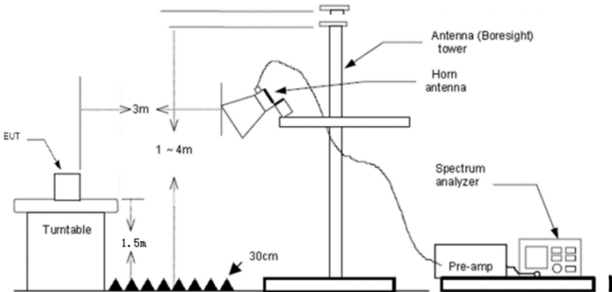
Figure 3. Above 1 GHz
