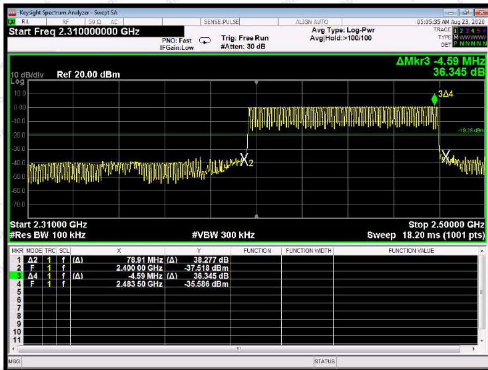
EDR mode-8DPSK
