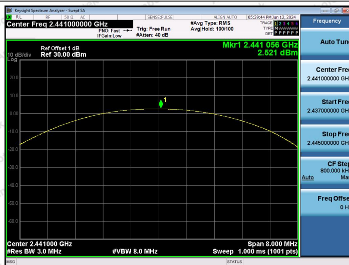
2.4G-Ant1-2441-PASS
