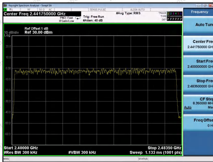
3DH5-Ant1-Hop-PASS
