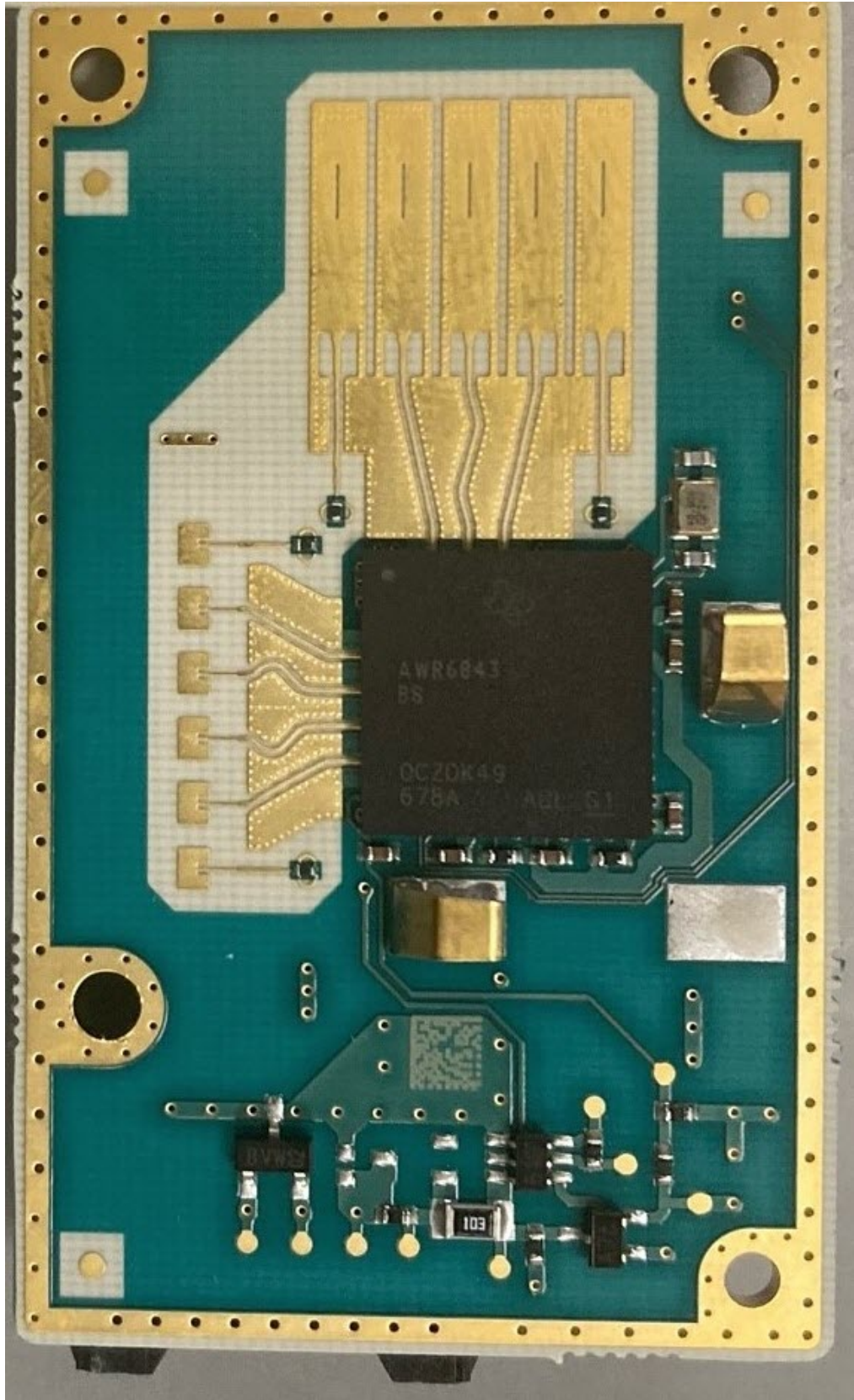
Figure 2: Bottom View
