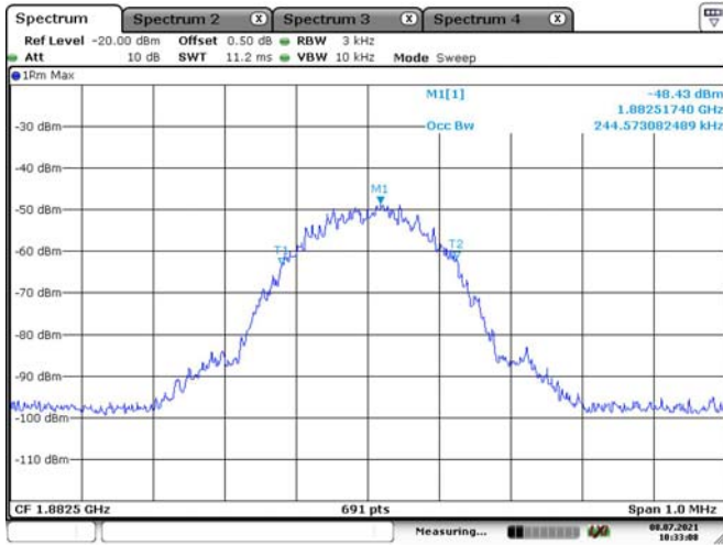
GSM-Input
