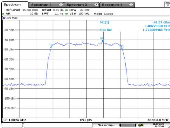
CDMA-Input
