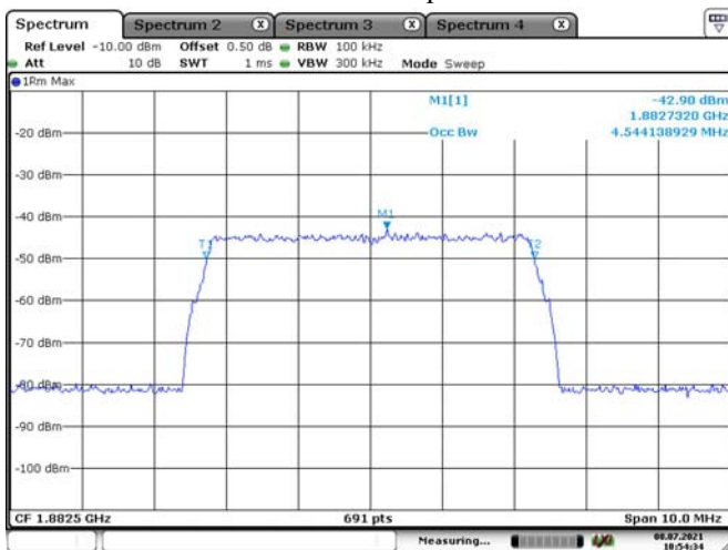
WCDMA-Input
