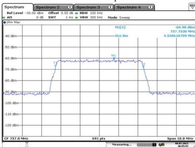
WCDMA-Input
