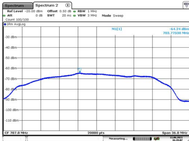
Lower 700M Band-Uplink
