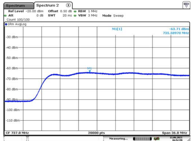
Lower 700M Band-Downlink
