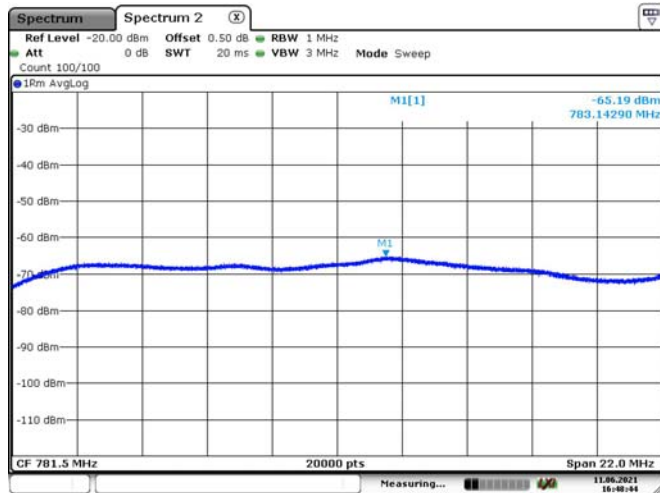
Upper 700M Band-Uplink
