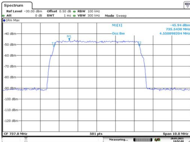
WCDMA-Input
