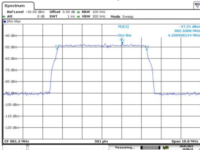
WCDMA-Input
