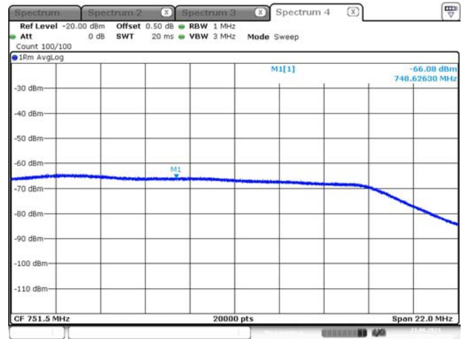
Upper 700M Band-Downlink
