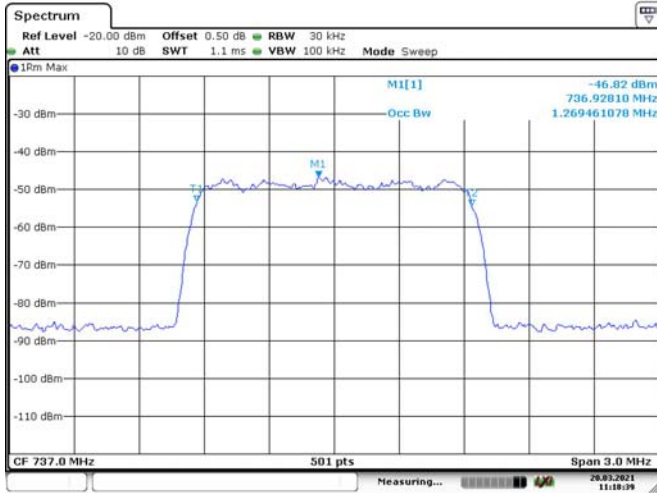
CDMA-Input
