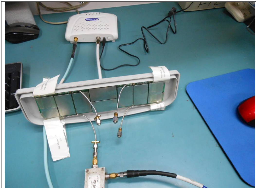
RF Conducted #2
