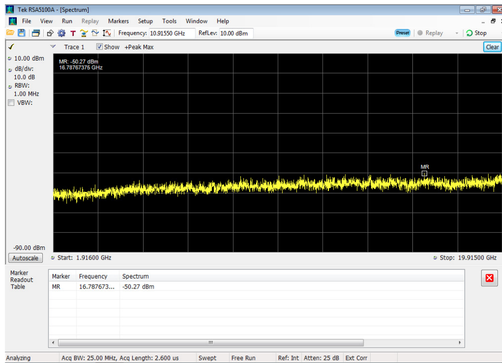
1850 - 1915 MHz_plot 2
