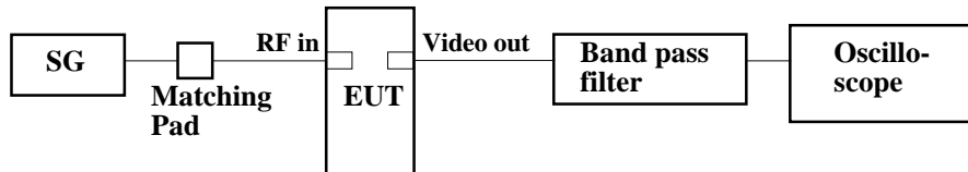
Figure 5. Picture sensitivity
